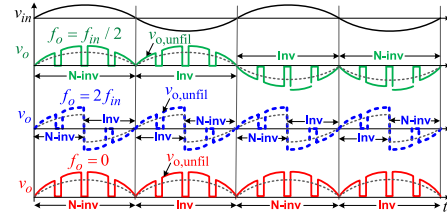
Fig. 16. Step-up/step-down frequency operation and ac-dc rectification.
