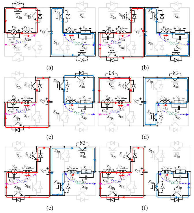
Fig. 12. Equivalent circuits for fNIBB operation when v_{in} > 0 : (a), (b) and (c) are for fNIBB operation, mode-I ( v_o > 0, i_o > 0 ); (a) D_a T and D_b T intervals. (b) D_a T and (1 - D_b)T intervals. (c) (1 - D_a)T and (1 - D_b)T intervals. (d), (e), and (f) are for fIBB operation, mode-II ( v_o < 0, i_o < 0 ); (d) D_a T and D_b T intervals. (e) D_a T and (1 - D_b)T intervals. (f) (1 - D_a)T and (1 - D_b)T intervals.
