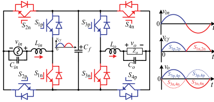
Fig. 3. Proposed high-efficiency buck–boost MC.
