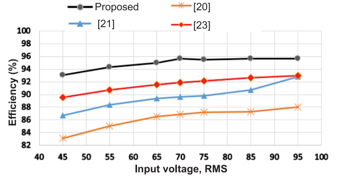
Fig. 33. Power conversion efficiency comparison for v_{in} = 45 \sim 95 V_{rms} .
