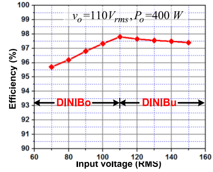
Fig. 32. Experimental efficiency of the proposed buck-boost MC for v_{in} = 70 \sim 150 V_{rms} .
