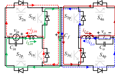
Fig. 15. Inductors L_{in} and L_o current flow paths during dead-time.
