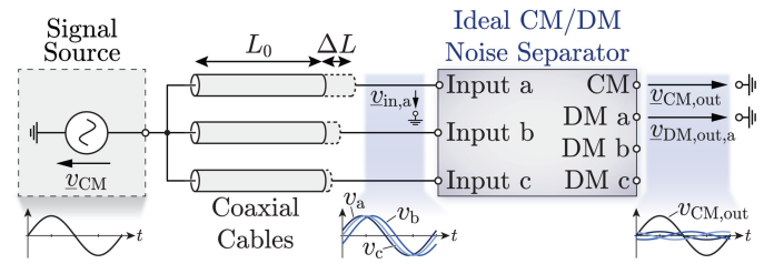
Fig. 11. Schematic representation of the CM-to-DM conversion introduced by connection cables with unequal length.
