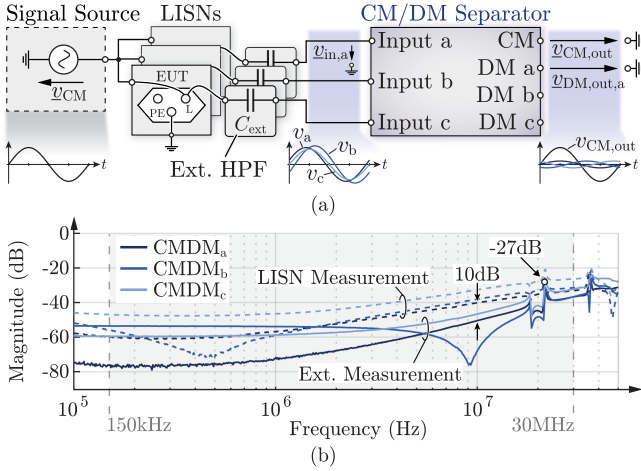
Fig. 15. (a) Extension of the LISN test setup with three external high-pass filters ( C_{ext} together with the separator input impedance) and (b) the resulting CM-to-DM conversion (continuous lines) in comparison with the direct LISN measurement (dashed lines) as presented before.
