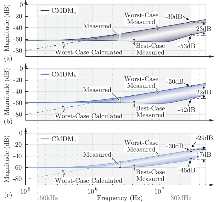
Fig. 12. Best- and worst-case CM-to-DM conversion measurements for all possible combinations of a cable mismatch at the noise separator inputs ( L_0 = 22 cm nominal cable length, length mismatch \Delta L = 4.8 cm). The calculated CM-to-DM conversion assuming an ideal noise separator is included for the worst-case length-mismatch configuration for each channel (dashed lines).
