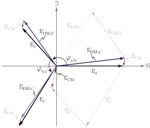
Fig. 5. Phasor diagram showing the decomposition of the three-phase voltage components into the respective CM and DM parts.
