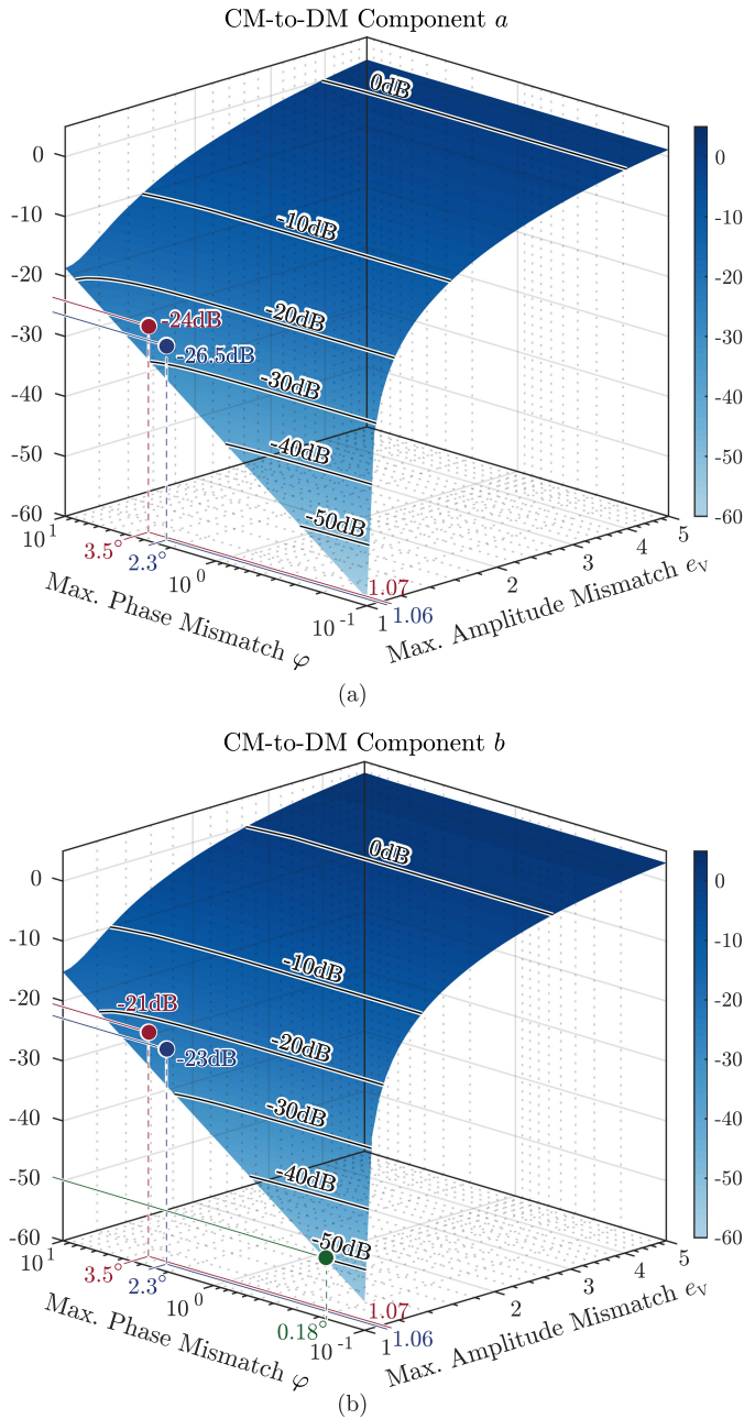
Fig. 10. Worst-case CM-to-DM conversions for DM component (a) a and (b) b considering all possible combinations of amplitude mismatches \{V_b/V_a, V_c/V_a\} \in [1/eV, eV] and phase mismatches \{\varphi_{ab}, \varphi_{ac}\} \in [-\varphi, \varphi] of inputs b and c assuming again input a as reference.
