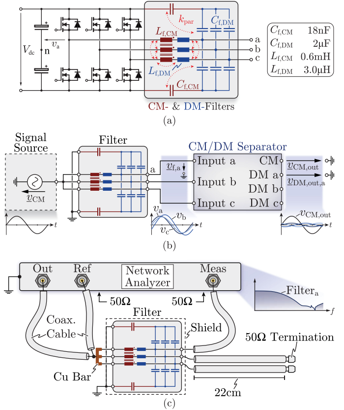
Fig. 16. (a) Three-phase inverter with a single-stage CM/DM output filter, where the components highlighted in red are solely responsible for CM filtering whereas the blue elements are primarily effective for DM filtering. (b) Configuration to measure the filter CM transfer function and the CM-to-DM conversion. (c) Measurement setup to characterize the individual phase filter transfer functions with a network analyzer.
