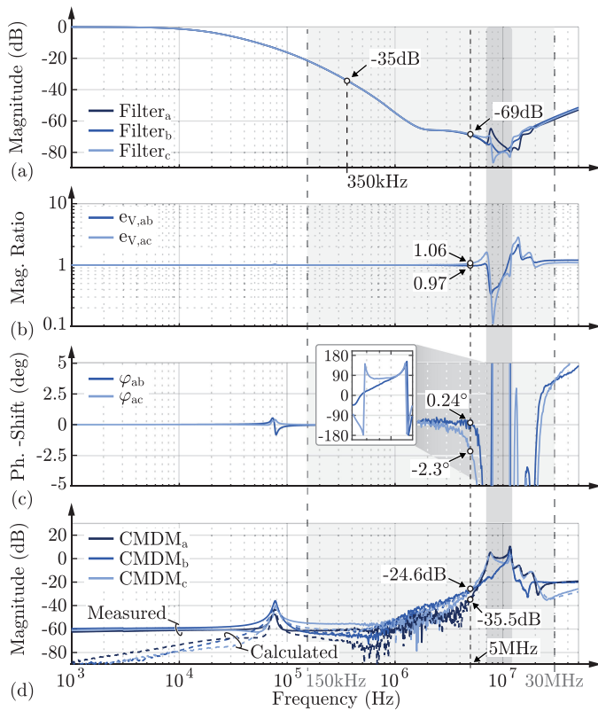
Fig. 17. (a) Measured filter CM transfer functions and therefrom (b) the calculated amplitude mismatches e_{V,ab} and e_{V,ac} and (c) the calculated phase mismatches \varphi_{ab} and \varphi_{ac} . (d) Calculated CM-to-DM conversion based on the amplitude and phase mismatches as well as the CM-to-DM conversion measured using an active three-phase noise separator.
