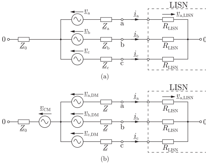
Fig. 18. (a) HF equivalent circuit of the three-phase converter with inner noise source impedances connected to the LISN and (b) decomposition into CM and DM parts.
