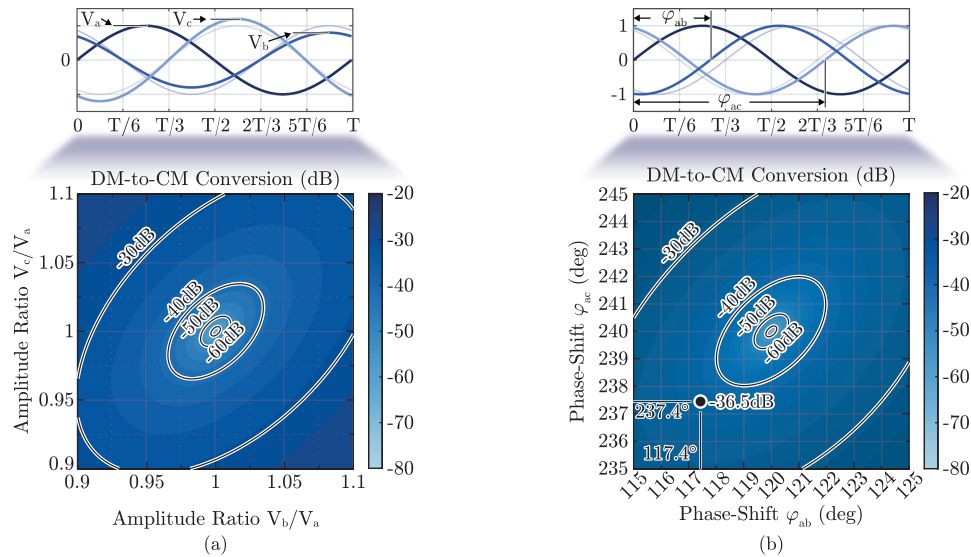
Fig. 19. Amplitude and phase mismatches at the output of an unsymmetric three-phase transmission system and related characterization of the transmission system with a DM-to-CM conversion under the assumption of a perfectly balanced three-phase DM input voltage system. For all cases, input channel a is treated as reference. (a) Considering only an amplitude mismatch V_b/V_a and V_c/V_a . (b) Considering only a phase mismatch \varphi_{ab} and \varphi_{ac} .
