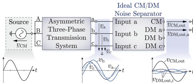
Fig. 8. Schematic representation of amplitude and phase mismatches in a asymmetric three-phase transmission system excited with a pure CM input voltage and the resulting CM-to-DM conversion.
