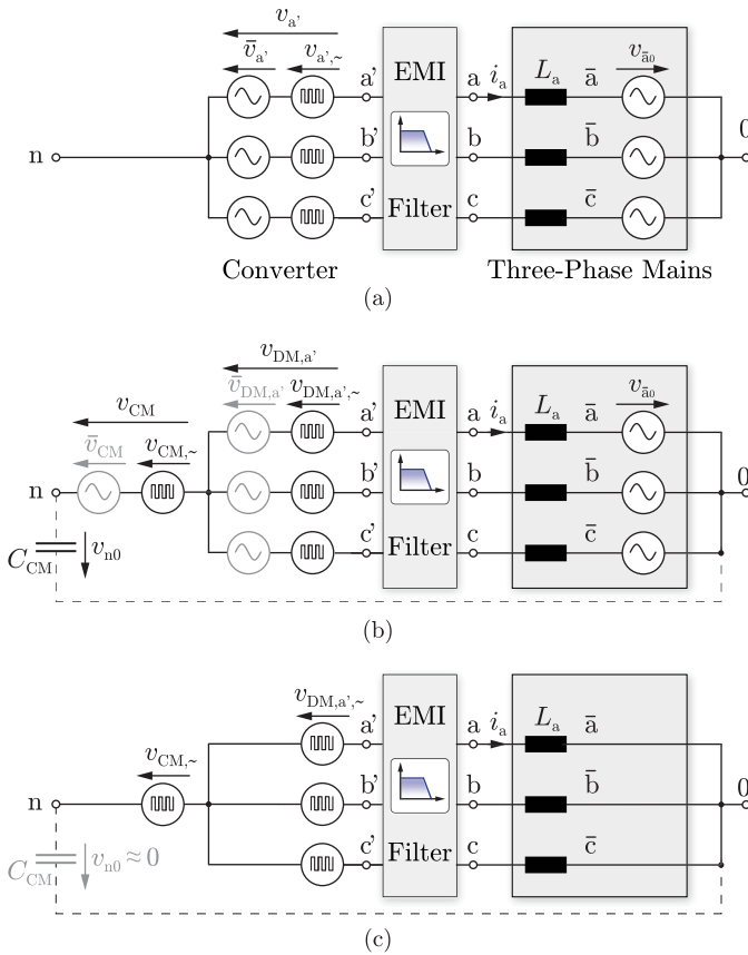
Fig. 4. Simplified representation of the three-phase inverter with EMI filter of Fig. 1 using equivalent voltage source circuits. (a) Three switch-node voltages v_{a'} , v_{b'} , and v_{c'} with a (desired) fundamental frequency component \bar{v}_i and a high-frequency switching component v_{i,\sim} and (b) further decomposition of both frequency components into CM and DM parts. (c) Only the EMI-relevant high-frequency components are considered for the worst-case with v_{n0} = 0 .
