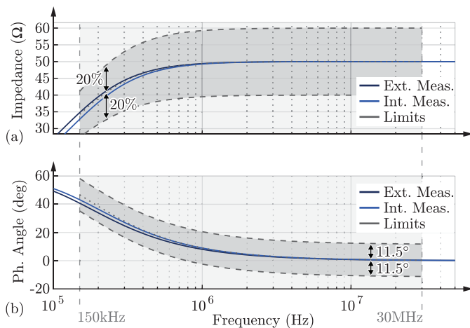
Fig. 20. LISN input impedance at the EUT port for both internal and external HF measurement paths. (a) Magnitude and (b) phase angle, including the tolerance band around the nominal value according to CISPR 16-1-2.
