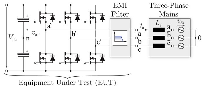
Fig. 1. Equipment under test (EUT): photovoltaic three-phase inverter system with output filter that supplies energy to the three-phase public mains (here shown with idealized sinusoidal voltage sources v_{i0} and corresponding inner mains inductances L_i , i \in \{a, b, c\} ).
