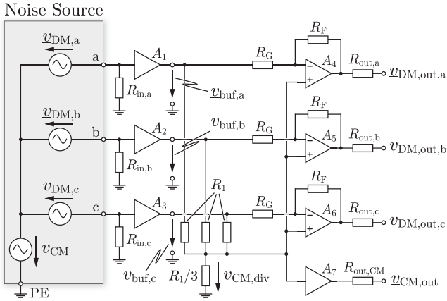
Fig. 6. Schematic drawing of an active three-phase CM/DM noise separator as described in [4].
