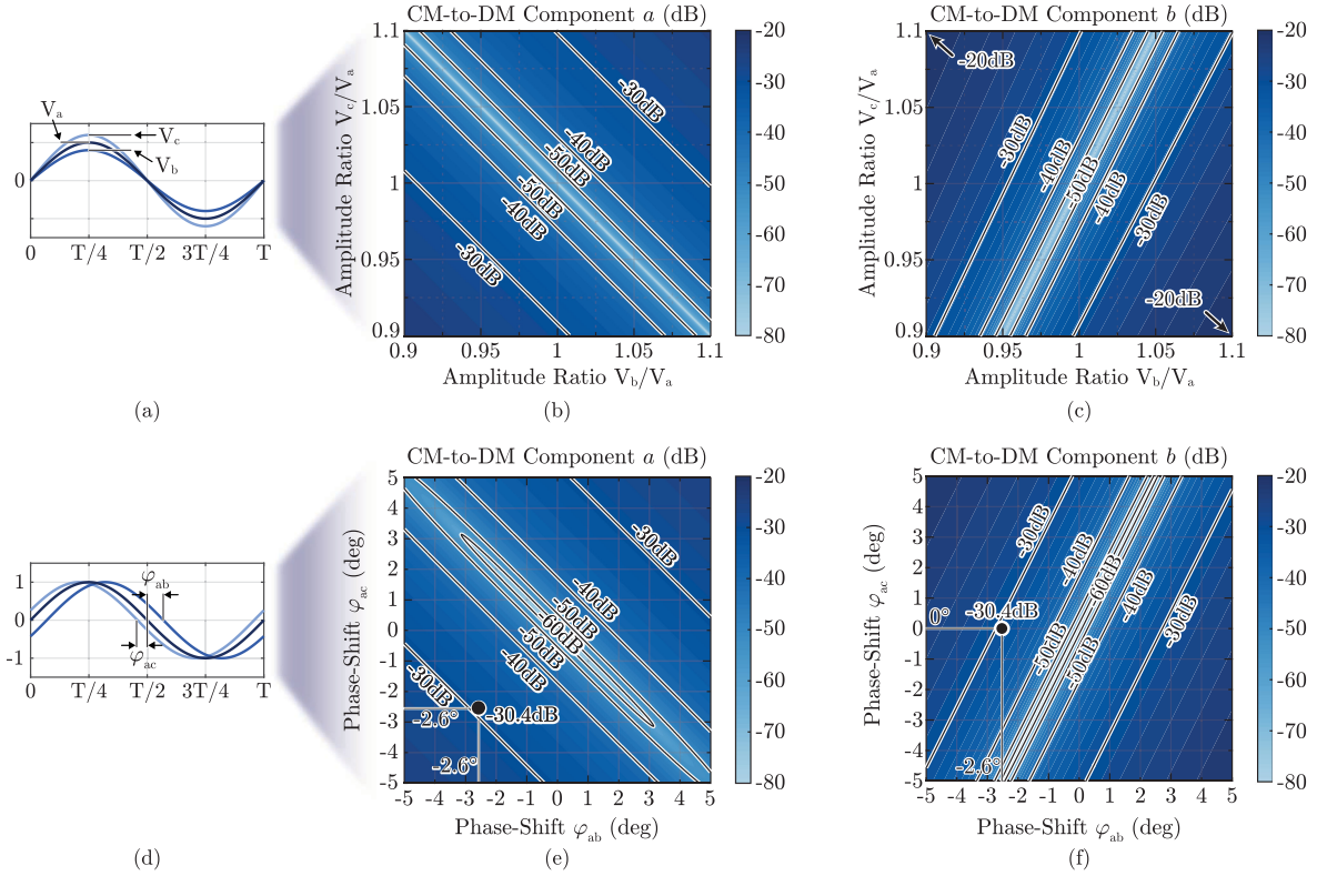
Fig. 9. Amplitude and phase mismatches at the output of an unsymmetric three-phase transmission system and related characterization with a CM-to-DM conversion. Input channel a is treated as reference, and input voltages b and c show amplitude/phase mismatches with respect to voltage a . (a)–(c) Considering only an amplitude mismatch V_b/V_a and V_c/V_a and (d)–(f) considering only a phase mismatch \varphi_{ab} and \varphi_{ac} .
