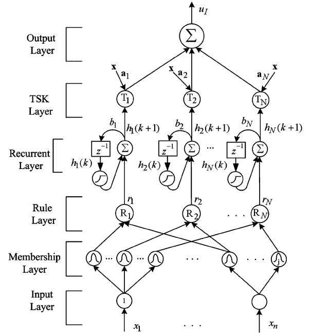
Fig. 12. RFNN controller for the high-precision trajectory tracking control of a linear microstepping motor driver [99]. A memory unit of time-delayed feedback connection Z^{-1} is added to enable the dynamic capability of NN controller.
