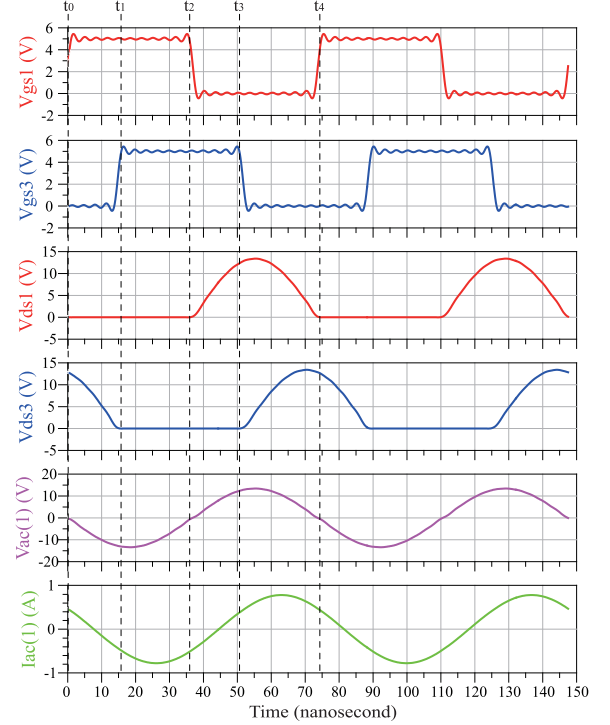
Fig. 9. Key waveforms of the cell-level balancer operating at 13.56 MHz.
