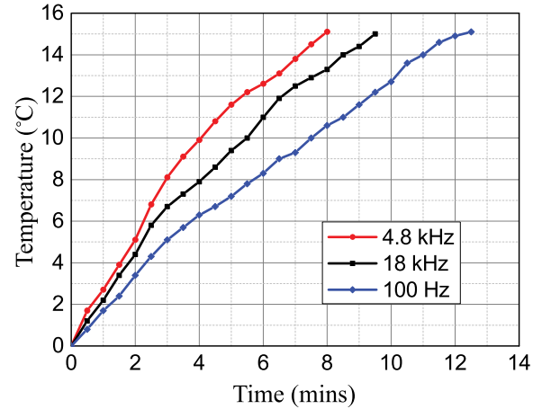
Fig. 21. Temperature rise of the battery strings in self-heating using current with different frequencies while maintaining the same voltage ripple \Delta V .
