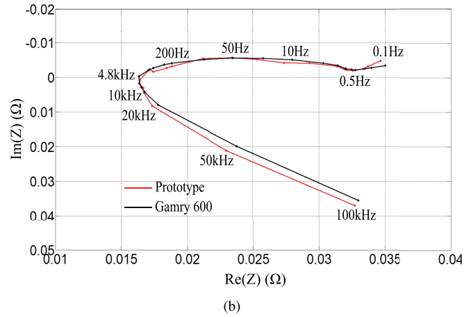
Fig. 19. (a) 10 kHz sinusoidal current generated by the 13.56-MHz CM Class-D converter for EIS measurement. (b) EIS measurement results of the prototype and a commercial instrument (Gamry Reference 600).
