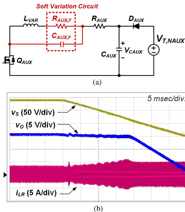
Fig. 10. Soft variation circuit during the transient. (a) Circuit diagram. (b) Mode transient waveform at 100% load conditions.
