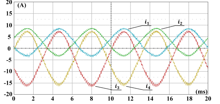
Fig. 11. M2dc-CT steady-state arm currents i_1 , i_2 , i_3 , and i_4 at P_{dc}^{\text{ref}} = 1.25 kW; experimental waveforms captured by oscilloscope.
