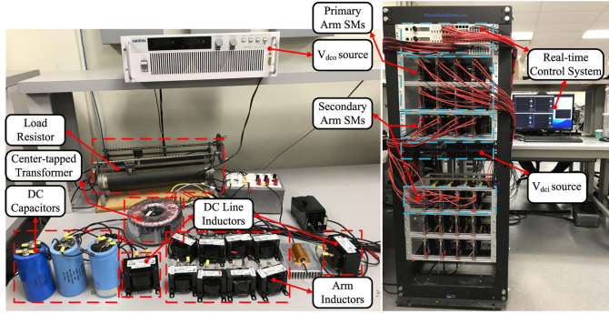
Fig. 8. M2dc-CT experimental setup.
