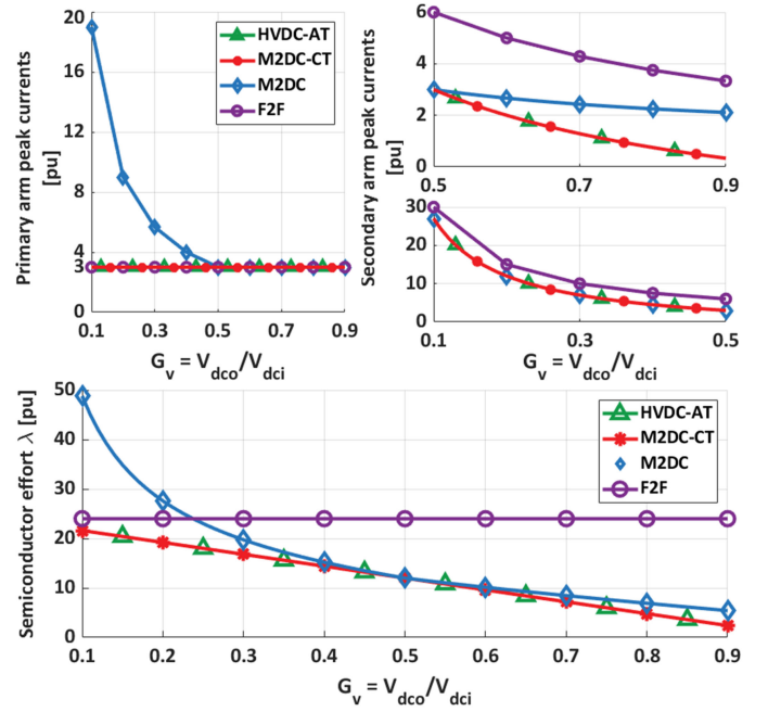
Fig. 14. Arms absolute peak current stresses, at rated power transfer and with maximum arm ac voltage utilization using half-bridge SMs (all currents are normalized to dc input current of each phase leg). Corresponding converter semiconductor efforts normalized to dc power transfer P_{dc} .
