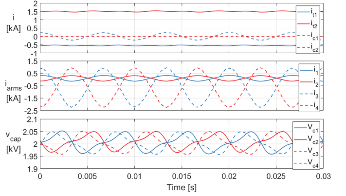
Fig. 6. Steady-state M2dc-CT current and voltage waveforms for G_v = 0.125 .
