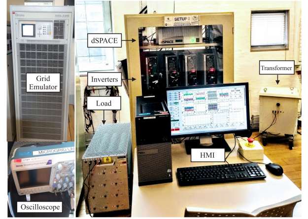
Fig. 5. Experimental setup formed by four inverters, voltage and current sensors, data acquisition, a dSPACE, human-machine interface, set of resistive loads, grid emulator, isolation transformer, and an oscilloscope.
