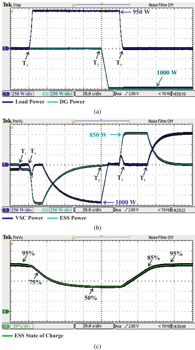
Fig. 6. Experimental results showing the power flow inside the dc microgrid. (a) In dark blue: load power consumption. In light blue: DG power supply. (b) In dark blue: VSC power. In light blue: ESS power for J = 1.0 , D_p = 1.0 . (c) Estimated ESS state of charge.
