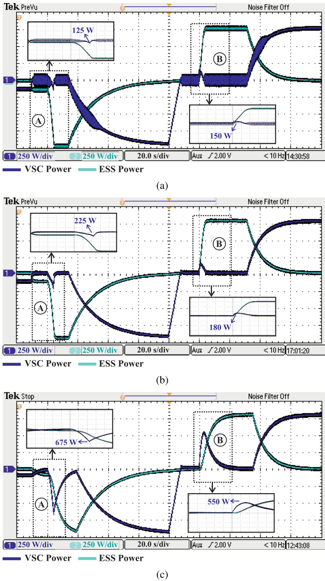
Fig. 7. Experimental results showing the power flow inside the dc microgrid when the parameter J is changed. In dark blue: VSC power. In light blue: ESS power. (a) J = 0.1 . (b) J = 0.5 . (c) J = 5.0 .
