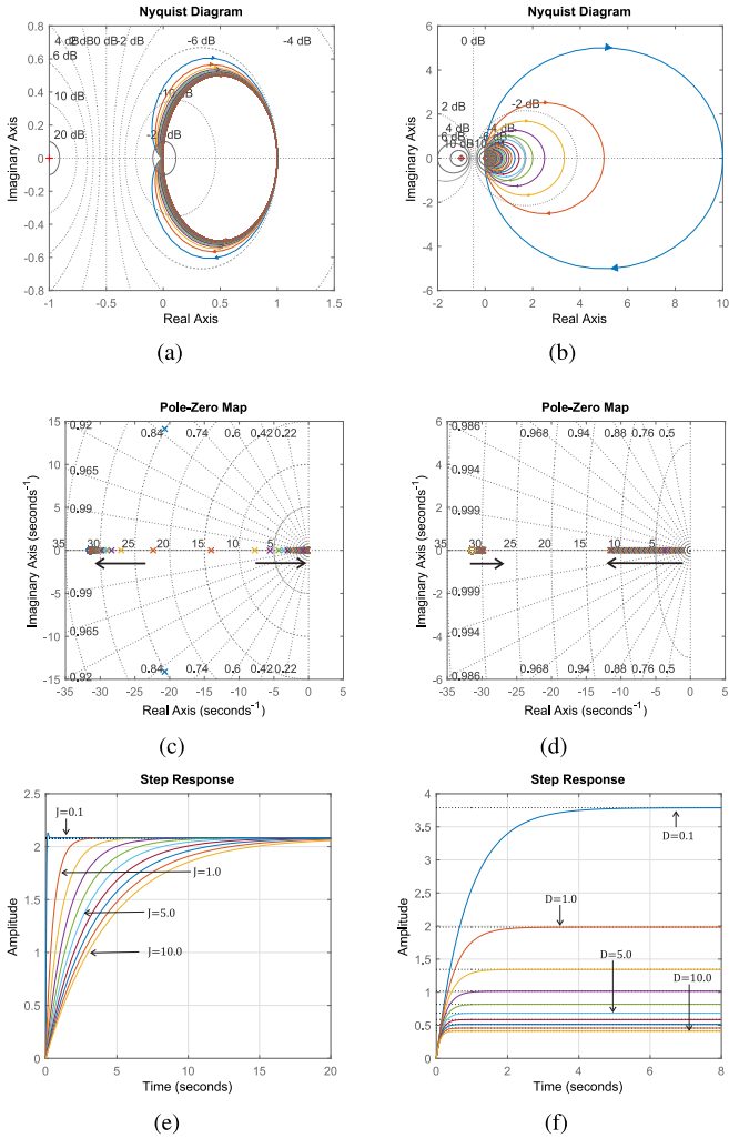
Fig. 4. PMS parameter variation analysis for J and D_p varying from 0.1 to 10. (a) Nyquist plot for J variation. (b) Nyquist plot for D_p variation. (c) Pole-zero mapping for J variation. (d) Pole-zero mapping for D_p variation. (e) 1-kW step response for J variation. (f) 1-kW step response for D_p variation.
