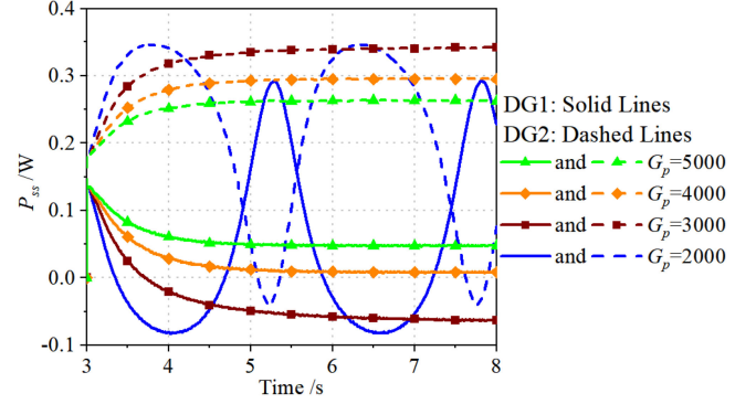
Fig. 20. Simulated waveforms of SACS real power for DG 1 and DG 2 under different amplification gains.
