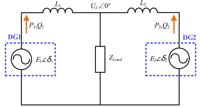
Fig. 3. Equivalent circuit of a two-DG-parallel islanded microgrid at fundamental frequency.
