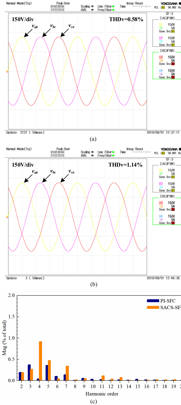
Fig. 27. PCC voltage waveforms under (a) PI-SFC, (b) SACS-SFC, and (c) THD analysis result.
