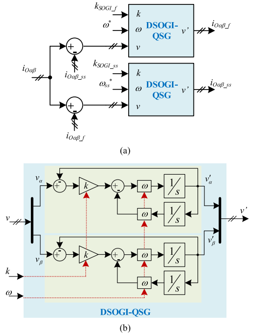
Fig. 9. Block diagram of (a) SOGI-based current signal extraction used in the proposed method and (b) DSOGI-QSG [40].
