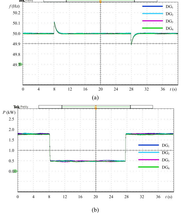
Fig. 26. Experimental waveforms of (a) frequency f and (b) output real power P of four DGs under the proposed SACS-SFC during load step changes.
