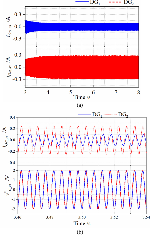
Fig. 19. Simulation waveforms of extracted SACS current and generated SACS voltage in both DGs: (a) extracted SACS current; and (b) zoomed-in waveform of SACS current and voltage.
