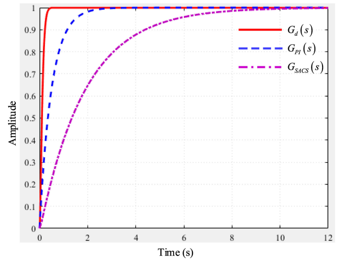
Fig. 16. Step response of primary droop control loop G_d(s) , PI control loop G_{PI}(s) , and SACS control loop G_{SACS}(s) .
