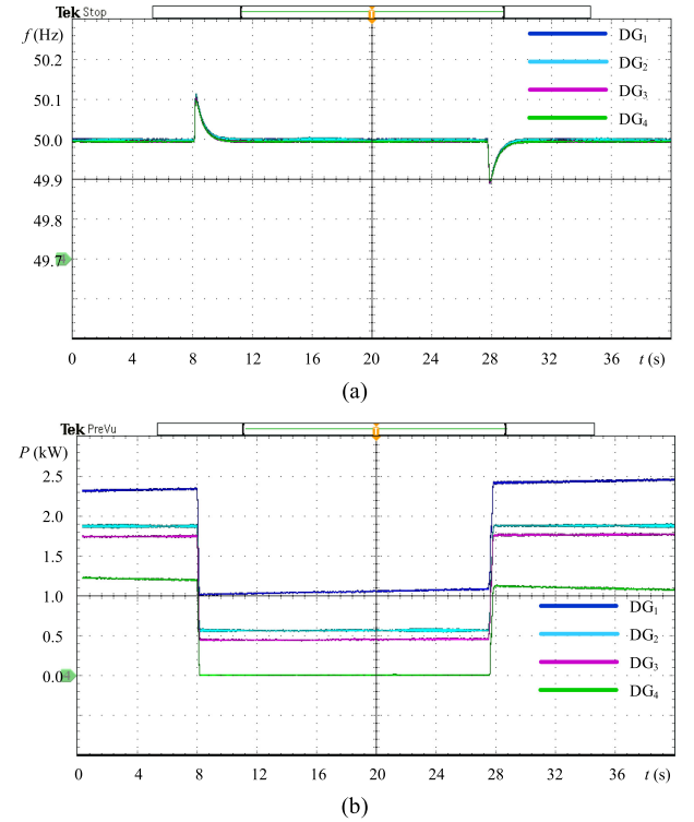
Fig. 25. Experimental waveforms of (a) frequency f and (b) output real power P of four DGs under PI-SFC during load step changes.
