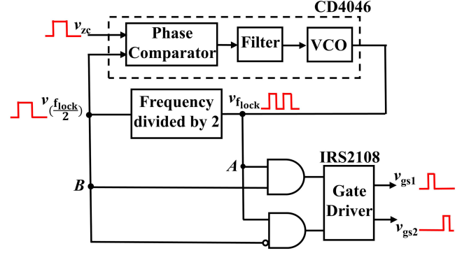
Fig. 10. PLL controller with frequency divider.
