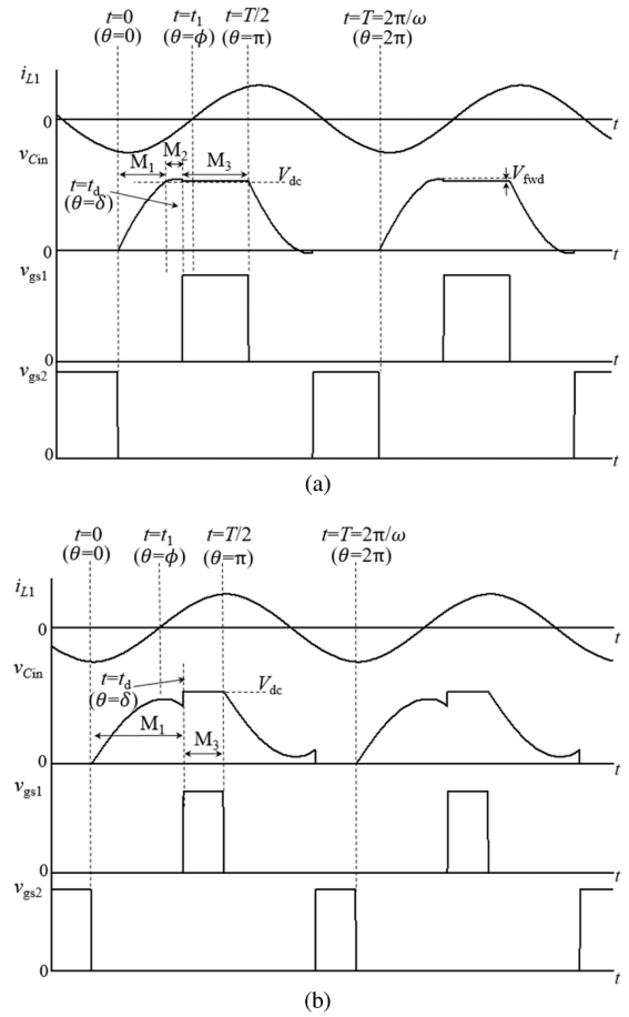
Fig. 2. Switching waveforms of the inductorless H-bridge PT-based converter. (a) ZVS achieved. (b) ZVS not achieved.
