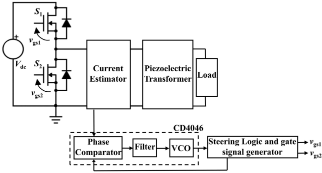
Fig. 3. Block diagram of the ZVS PLL control system.
