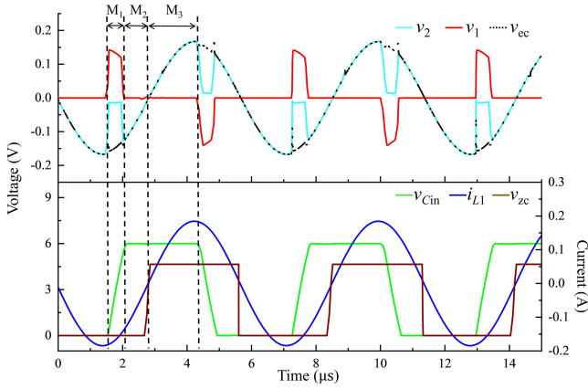
Fig. 5. Operating waveforms of current estimator 1.
