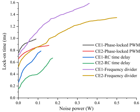
Fig. 13. Lock-on time comparison of the proposed PLL controllers associated with current estimator 1 (CE1) and current estimator 2 (CE2) under noise condition.
