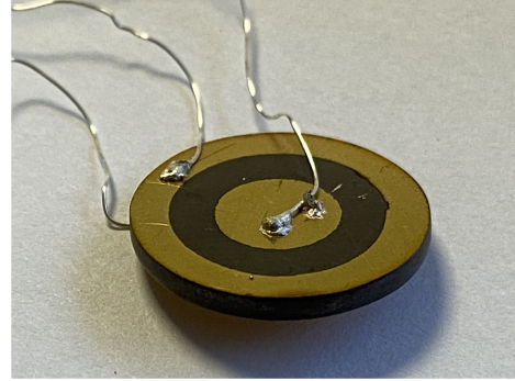
Fig. 11. Ring-dot radial-mode PT under test.
