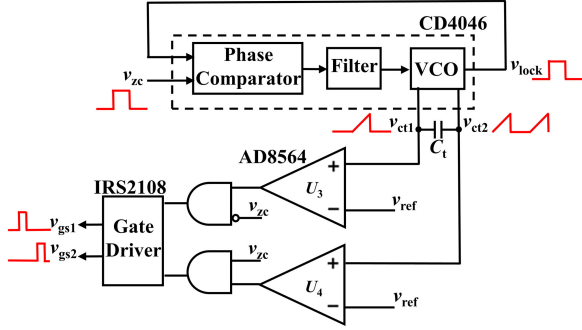
Fig. 8. PLL controller with phase-locked PWM.
