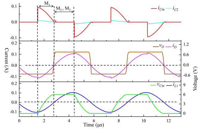
Fig. 7. Operating waveforms of current estimator 2.
