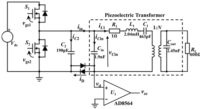
Fig. 6. Current estimator 2 (the antiparallel diode sign detector).
