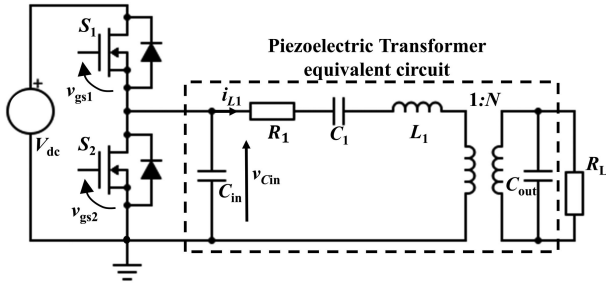
Fig. 1. Inductorless H-bridge PT-based converter with Mason equivalent circuit.
