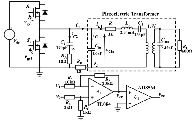
Fig. 4. Current estimator 1 (the voltage differentiator).
