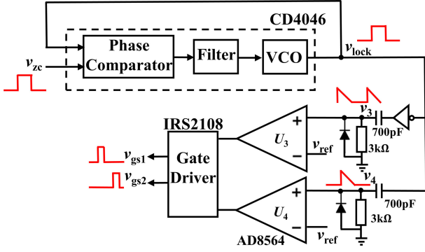
Fig. 9. PLL controller with RC time delay.
