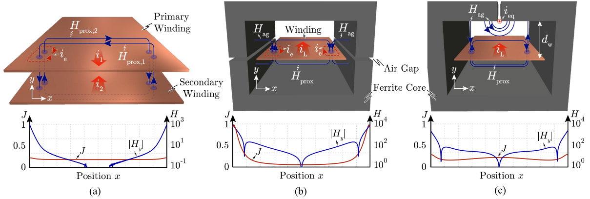
Fig. 3. Magnetic field distributions and the corresponding normalized current densities J and vertical magnetic field components H_y . (a) PCB-winding transformer with coplanar arrangement of the two windings. (b) Conventional PCB-winding inductor with the air gap in the same physical layer as the winding. (c) Proposed PCB-winding inductor design, where the air gap is arranged perpendicularly to the windings.
