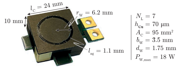
Fig. 24. Practically implemented 6.8\mu\text{H} PCB-winding inductor with a CNC-milled ferrite core made out of N49 material.
