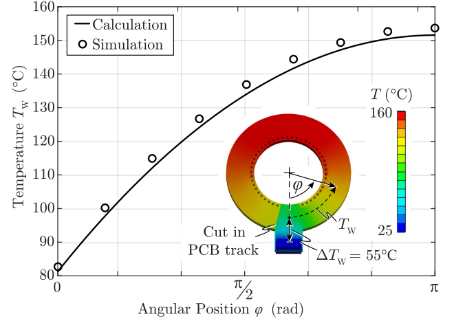
Fig. 15. Temperature profile for the PCB winding shown in Figs. 9 and 14 for 6 W of total losses. Additionally, the corresponding FEM simulation is shown.
