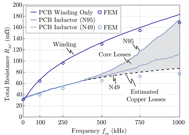
Fig. 10. Total winding resistance of the PCB winding only (air coil), the fully assembled inductor with a core made of N95, and the same inductor but with a core made of N49 ferrite material. All three measurements were taken using an impedance analyzer.
