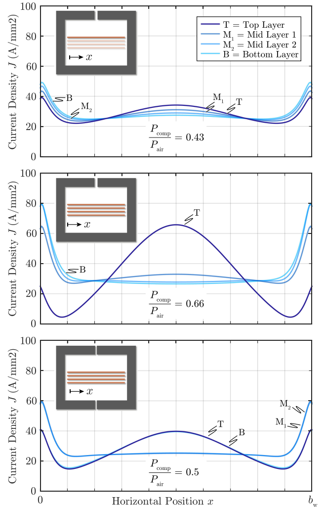
Fig. 8. Simulated current densities in a four-layer PCB. (a) Single air gap and all layers simulated independently from each other, one at a time (neglecting the proximity effect). (b) Single air gap and all layers simulated simultaneously (real situation). (c) Dual air gap arrangement with simultaneously simulated PCB layers. Additionally, the occurring conduction losses are always compared to the one arising in the PCB without a magnetic core (air coil).
