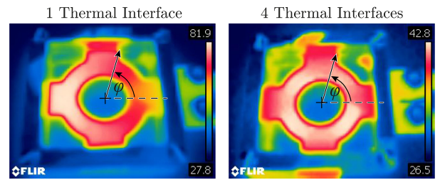
Fig. 19. Calculated thermal profiles of the inductors shown in Fig. 18, for total winding losses of 3.5 W. Additionally, the corresponding thermal images of the measured inductors are shown for the same amount of losses.
