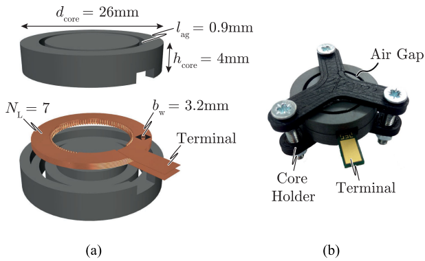
Fig. 9. (a) 3-D model of the practical implementation of a 6.8- \mu H multilayer PCB-winding inductor using the proposed field compensation concept, by means of a ferrite core with two air gaps and (b) picture of the assembled inductor with a 3-D-printed core holder.
