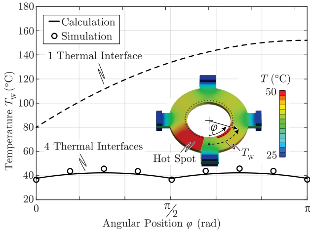
Fig. 17. Temperature profile of the thermally enhanced PCB winding (four thermal interfaces) for 6 W of total losses. Additionally, the corresponding FEM simulation is shown.
