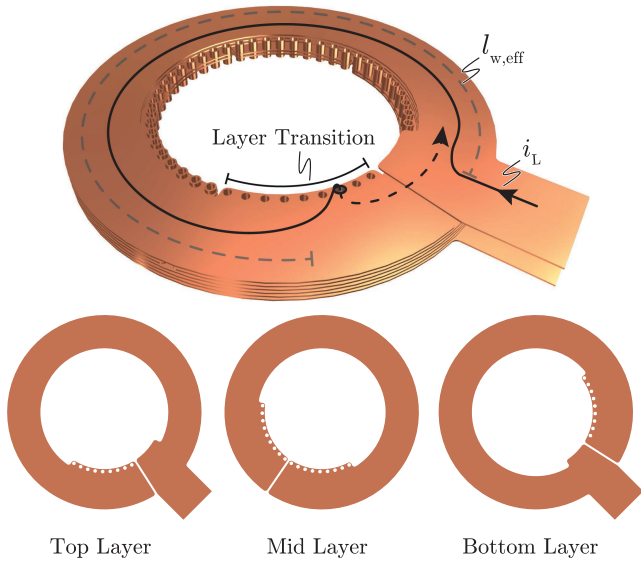
Fig. 6. Design of a multilayer PCB winding with single turns on each layer and through-hole vias for the transitions between the layers and/or interconnections of the turns. Additionally, the shapes of the different copper layers are shown, where it needs to be mentioned, that all the inner layers (Mid Layer) look the same just rotated by a certain rotation angle, which is why it is shown only once.
