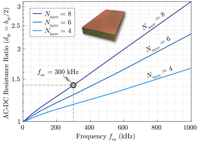
Fig. 21. AC to dc resistance ratios of inductor windings implemented in four-, six-, and eight-layer PCBs for an air gap placement according to (1).
