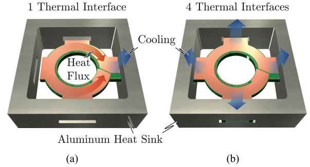
Fig. 18. Experimental test setups. (a) PCB winding with only a one thermal interface at the electric winding terminals. (b) Same winding but with four thermal interfaces.
