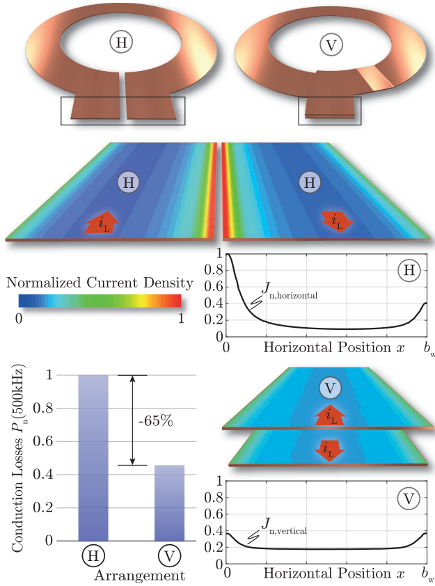
Fig. 7. FEM-simulated current densities in a horizontal \textcircled{H} and a vertical \textcircled{V} parallel termination for a frequency of 500 kHz and a track width of 5 mm. The normalized conduction losses P_n of the two possible terminations are also shown.
