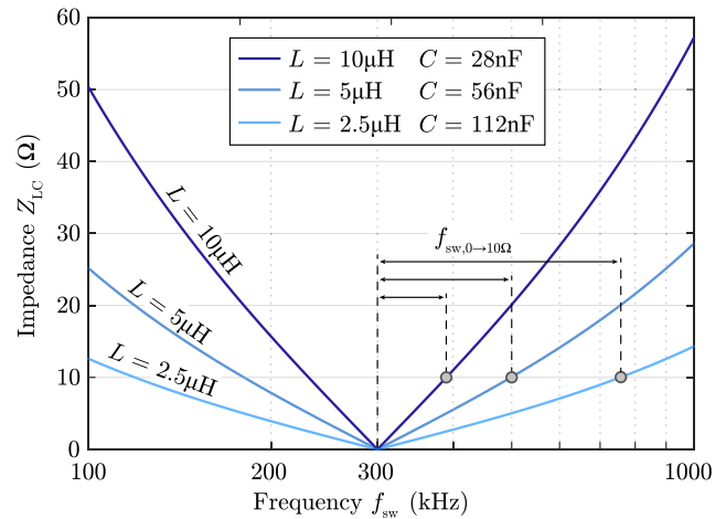
Fig. 2. Three impedance curves of different resonant tanks with the same resonance frequency of 300 kHz are shown. Additionally, the required frequency range f_{sw,0 \rightarrow 10\Omega} for an increase of the tank impedance Z_{LC} from 0 to 10 \Omega is illustrated.
