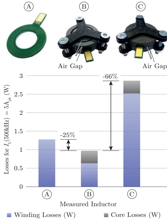
Fig. 11. Calorimetric loss measurements of (A) the PCB winding only, with an inductance of 700 nH, (B) the proposed PCB-winding inductor design (N49) with an inductance of 6.7 \mu H and (C) the conventional design approach with the air gap in the same physical layer as the PCB (6.8 \mu H).
