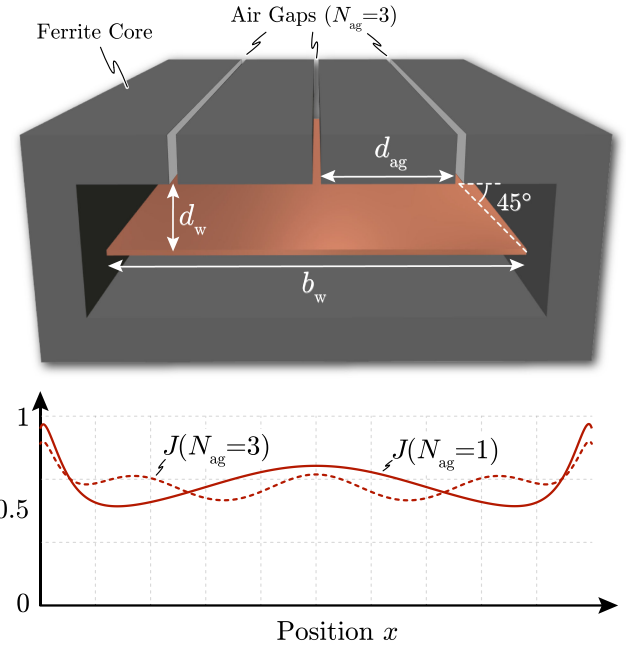
Fig. 5. Optimal arrangement of a PCB-winding inductor with three air gaps. The cutting surfaces of the core are colored in light gray in order to ensure good visibility of the air gap placement. In addition, the normalized current density distribution of a single air gap ( N_{ag} = 1 ) and triple air gap ( N_{ag} = 3 ) arrangement are shown.
