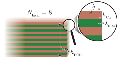
Fig. 12. Sketch of an eight-layer PCB with all the definitions used to introduce an effective thermal conductivity \lambda_{eff} of a PCB [cf. (3–5)].
