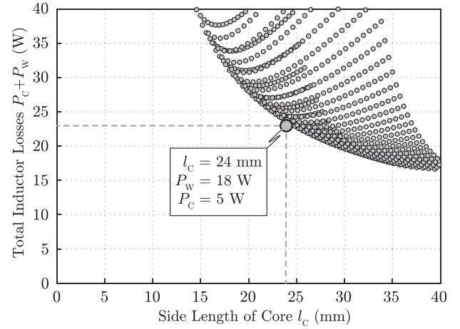
Fig. 23. Pareto optimization of a PCB-winding inductor according to the specifications given in Table II. Additionally, the chosen design is shown with its loss composition and the side length of the ferrite core.
