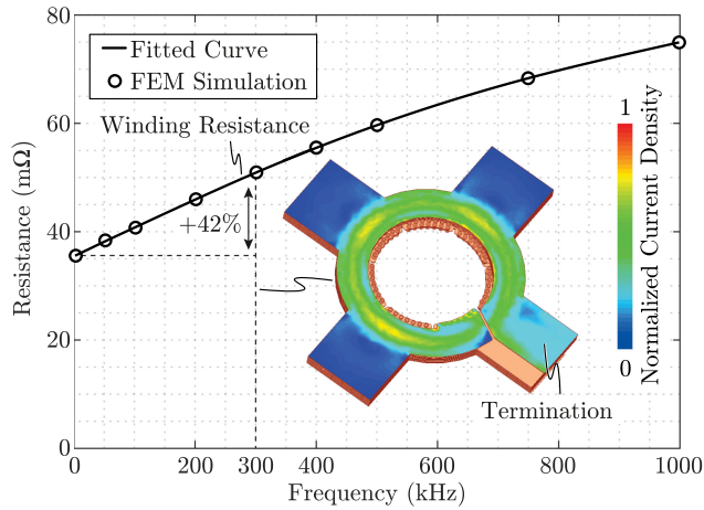
Fig. 25. FEM-simulated winding resistance of the PCB-winding inductor shown in Fig. 24 and the corresponding normalized current density distribution at 300 kHz.
