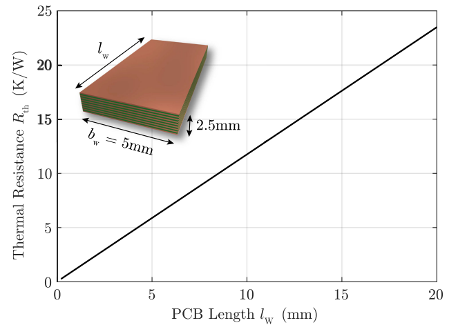
Fig. 13. Thermal resistance of a piece of an eight-layer 70 \mu m PCB with a width of 5 mm, a height of 2.5 mm, and a variable length l_w .
