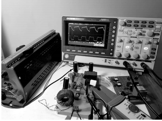
Fig. 15. Experimental setup of the proposed CIBuBoC.
