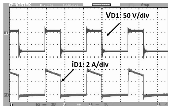
Fig. 19. Experimental waveforms for switch D_1 in step-up mode.
