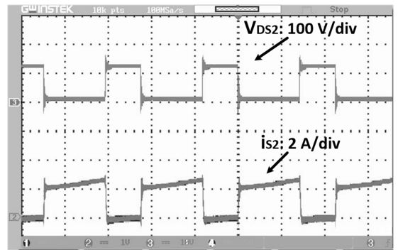
Fig. 18. Experimental waveforms for switch S_2 in step-up mode.
