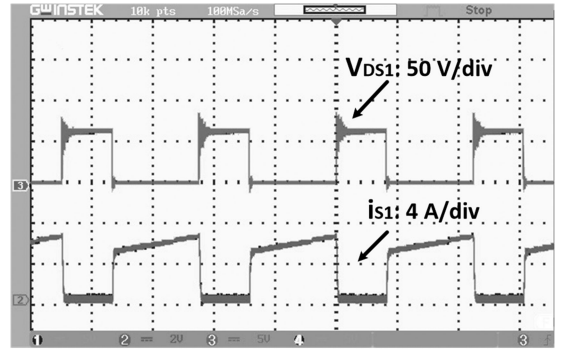
Fig. 17. Experimental waveforms for switch S_1 in step-up mode.
