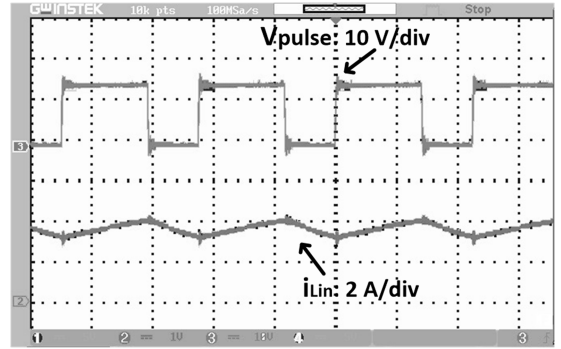
Fig. 16. Measured MOSFETS gate voltage and input inductor current i_{L1} in step-up mode.
