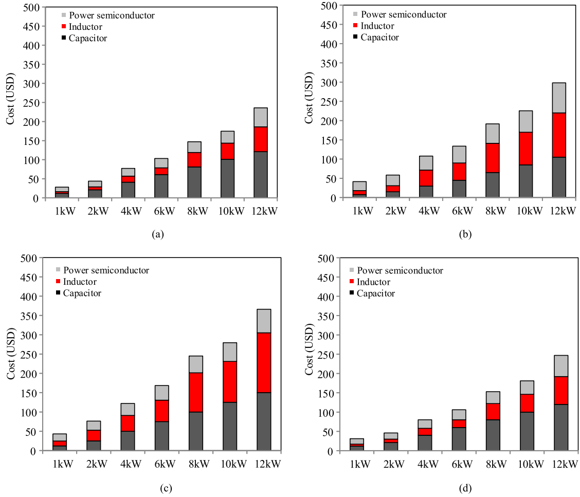
Fig. 20. Cost evaluate results of the four cases with ten years lifetime target and scalable power rating. (a) Cost of passive solution with a scalable power rating. (b) Cost of 1A solution with a scalable power rating. (c) Cost of 6A solution with a scalable power rating. (d) Cost of 42F solution with a scalable power rating.
