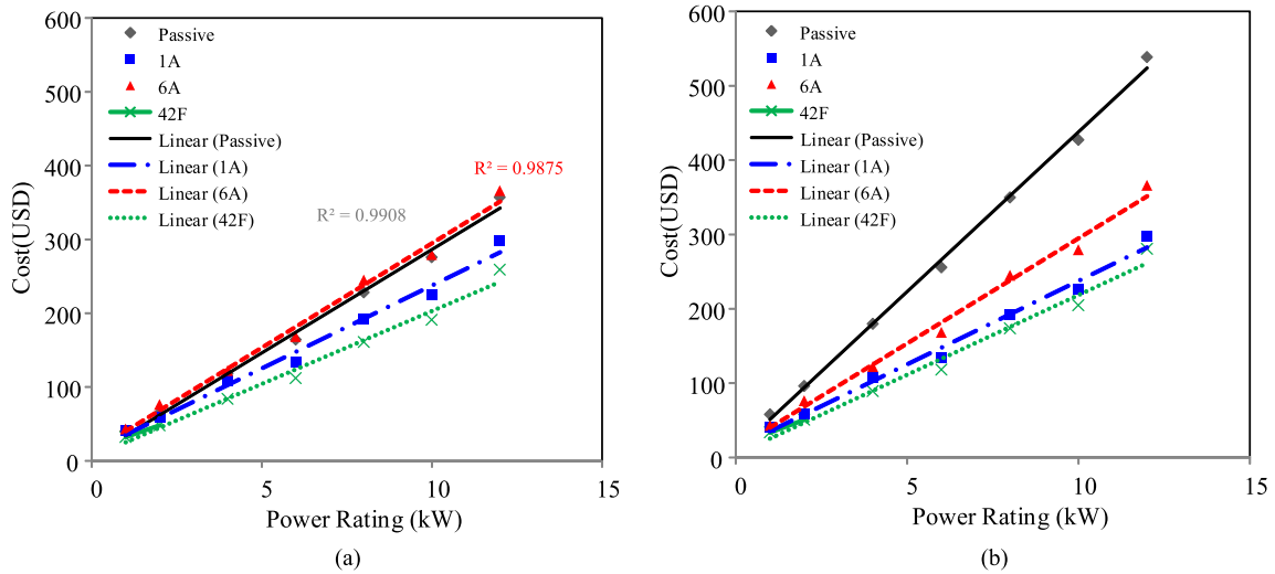
Fig. 21. Cost evaluate results of four cases with 20 and 35 years lifetime target and scalable power rating. (a) With 20 years lifetime target. (b) With 35 years lifetime target.
