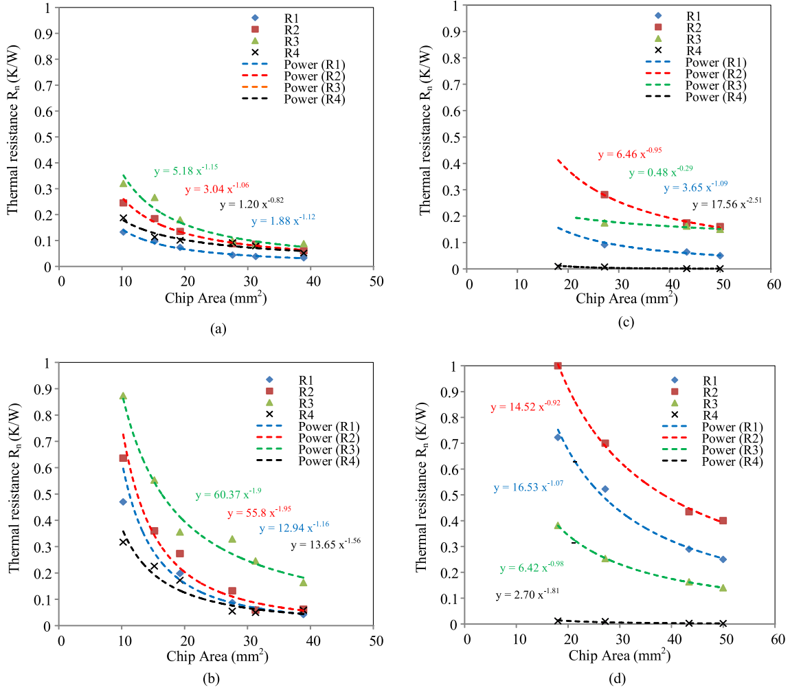
Fig. 11. Curve fitting results of thermal impedance parameters to the selected power devices. (a) Thermal resistance of 600 V transistor. (b) Thermal resistance of 600 V diode. (c) Thermal resistance of 1200 V transistor. (d) Thermal resistance of 1200 V diode.
