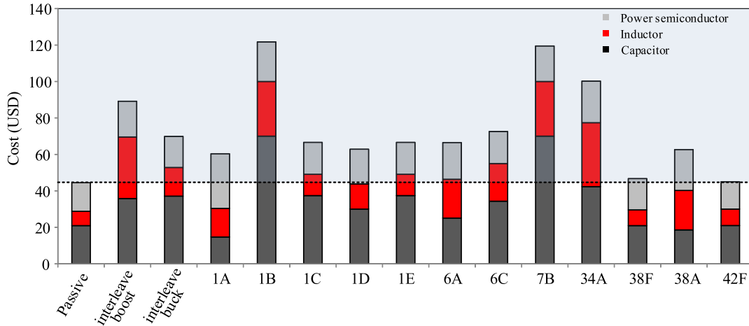
Fig. 16. Total cost of capacitors, inductors, and power devices of the existing methods with ten years lifetime target.
