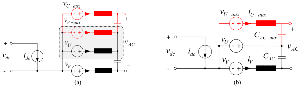
Fig. 6. Average model of the example of synthesis optimization. (a) Synthesis topologies based on full-bridge converters. (b) Synthesis optimization.
