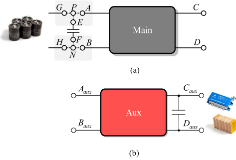
Fig. 2. Basic module for the main circuit and the auxiliary circuit. (a) Main circuit. (b) Auxiliary circuit.
