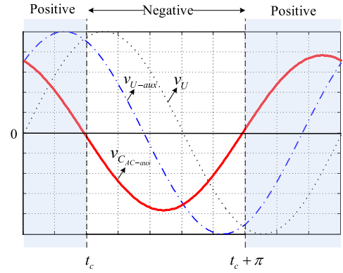
Fig. 23. Modulation waveforms for each two legs in one fundamental frequency.
