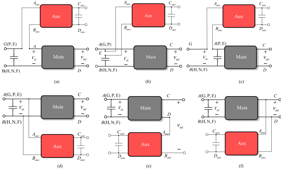
Fig. 3. Structure diagrams of the auxiliary circuit connected with the main circuit. (a) Connect the auxiliary circuit in series with the dc side of the main circuit (converter side). (b) Connect the auxiliary circuit in series with the dc side of the main circuit (capacitor side). (c) Connect the auxiliary circuit in series with the dc side of the main circuit (input side). (d) Connect the auxiliary circuit in parallel with the dc side of the main circuit. (e) Connect the auxiliary circuit in series with the ac side of the main circuit. (f) Connect the auxiliary circuit in parallel with the ac side of the main circuit.
