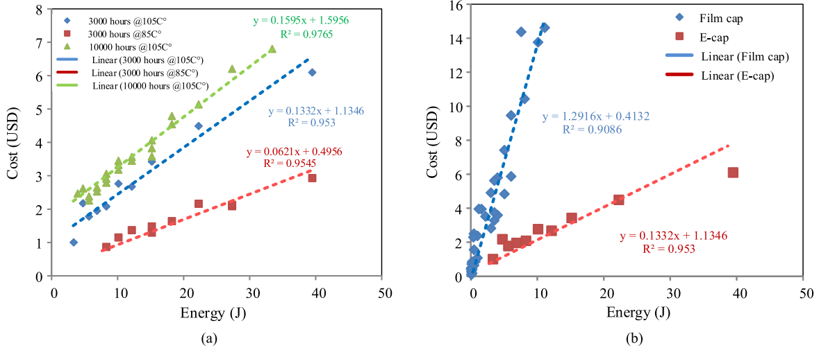
Fig. 15. Statistical results of a unit cost of different kinds of capacitors, which are represented as a unit price for 1000 pieces ordering quantity (source: [123]). (a) Cost models of different types of E-caps. (b) Cost models of 3000 hours @105° E-cap and film capacitors.
