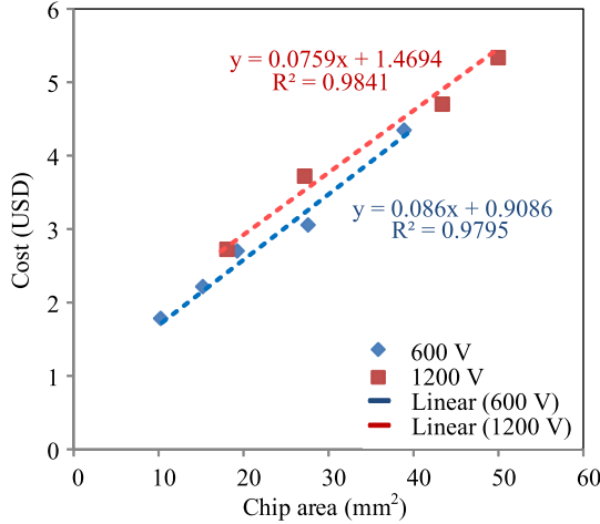
Fig. 14. Statistical results of a power semiconductor cost, which is represented as a unit price for 1000 pieces ordering quantity (source: [122], [123]).
