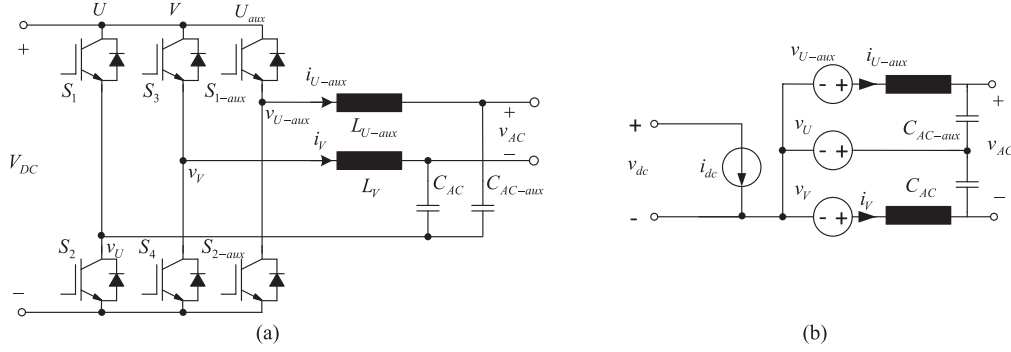
Fig. 13. Three legs single-phase structure used for the inductor design and analysis. (a) Topology used for inductor design. (b) Average model of the topology used for inductor design.
