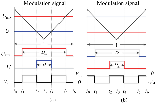
Fig. 24. Switching sequences of each two legs in one switching period. (a) v_s is positive. (b) v_s is negative.
