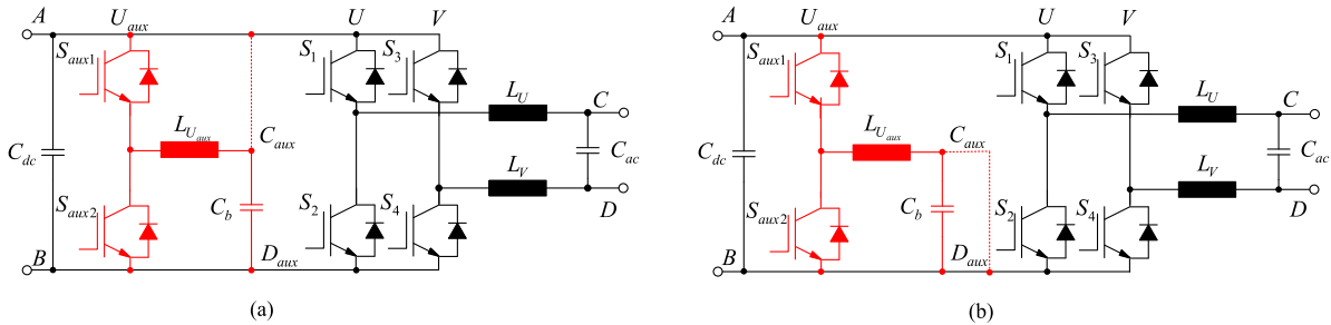
Fig. 7. Two topology examples that do not work following the principle in synthesis procedure. (a) Switch short circuited. (b) Capacitor short circuited.
