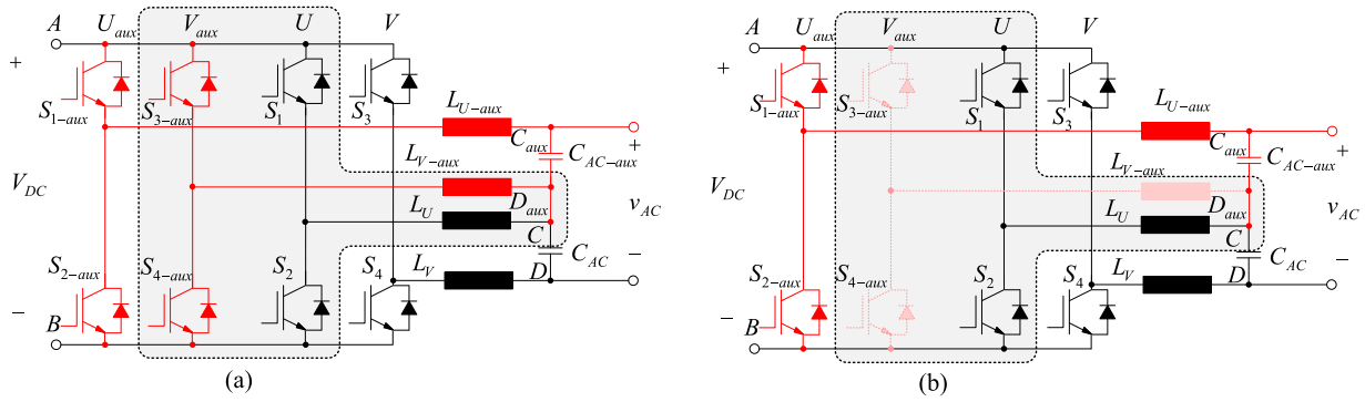
Fig. 5. Example of synthesis optimization based on full-bridge converters. (a) Synthesis topologies based on full-bridge converters. (b) Synthesis optimization.
