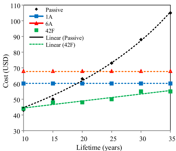
Fig. 19. Relation between the lifetime target and cost of four cases.
