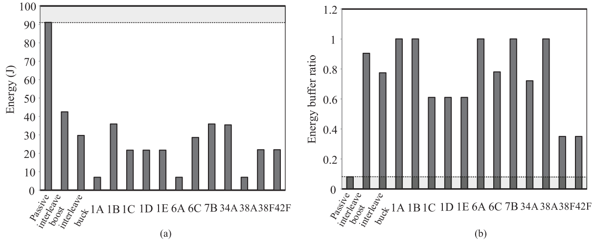
Fig. 22. Total energy stored in capacitors and energy buffer ratio comparisons among typical active dc-link solutions. (a) Total energy stored in capacitors of key solutions. (b) Energy buffer ratio of key solutions.
