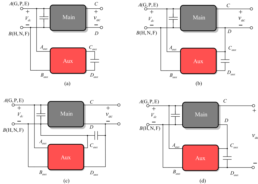
Fig. 4. Synthesis modes for the dc parallel case shown in Fig. 3 (d). (a) Hang mode. (b) Float mode. (c) Parallel mode. (d) Series mode.
