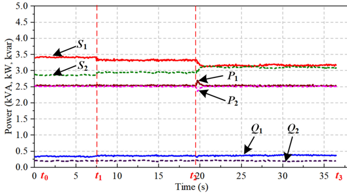
Fig. 24. Experimental waveforms of output apparent power, active power, and reactive power of DG1 and DG2 under the traditional droop method, the direct droop method, and the proposed control method.
