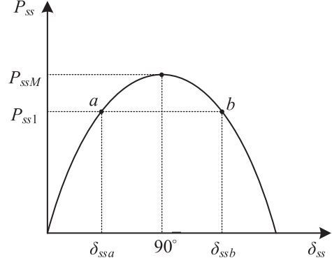
Fig. 11. Variation of active power with phase angle in each DG unit at the frequency of injected SACS.
