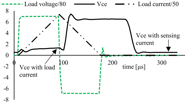
Fig. 10. Measurements within a switching period of the proposed cycle.
