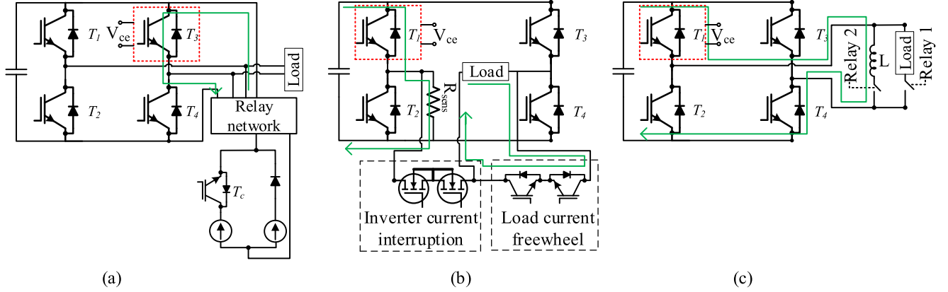
Fig. 2. Power circuits for aging detection of IGBT modules using the V_{ce} method with sensing or load current, the enclosed IGBT in the red-dashed square is the DUT. (a) Power circuit with additional high-current source and relays for the V_{ce} method with sensing and load current [2]. (b) Power circuit with current redirection for the V_{ce} method with sensing and load current [13]. (c) Power circuit with test inductor only for the V_{ce} method with load current in the ZTC operating region [15].
