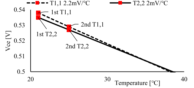
Fig. 6. Thermal characterization of IGBT modules at sensing current with and without water flow in the cooling plate.
