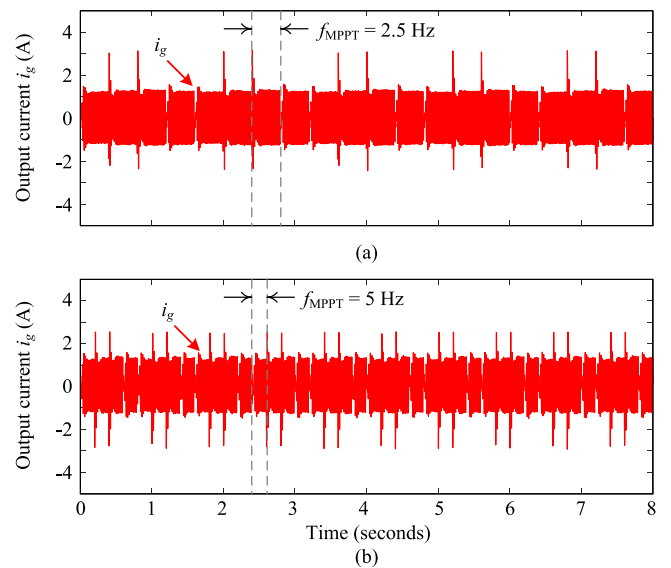
Fig. 3. Experimental waveforms of the output current i_g of the PV inverter operated at 10% of the rated power (i.e., 0.3 kW) with the MPPT sampling rate of (a) f_{MPPT} = 2.5 \text{ Hz} and (b) f_{MPPT} = 5 \text{ Hz} .
