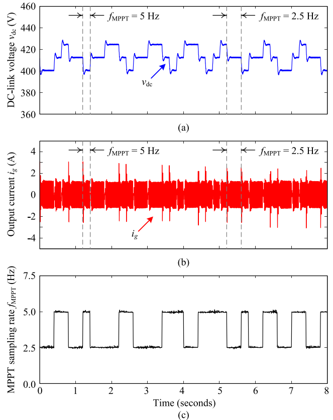
Fig. 5. Experimental results of the PV inverter operated at 10% of the rated power (i.e., 0.3 kW) with randomly applied MPPT sampling rate of f_{slow} = 2.5 Hz and f_{fast} = 5 Hz. (a) DC-link voltage v_{dc} . (b) Output current i_g . (c) MPPT sampling rate f_{MPPT} .
