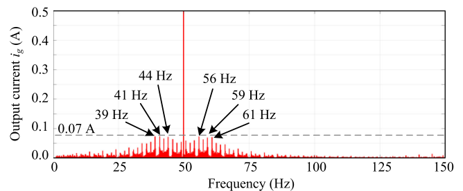
Fig. 6. Frequency spectrum of the output current i_g of the PV inverter operated at 10% of the rated power (i.e., 0.3 kW) with randomly applied MPPT sampling rate of f_{slow} = 2.5 Hz and f_{fast} = 5 Hz.
