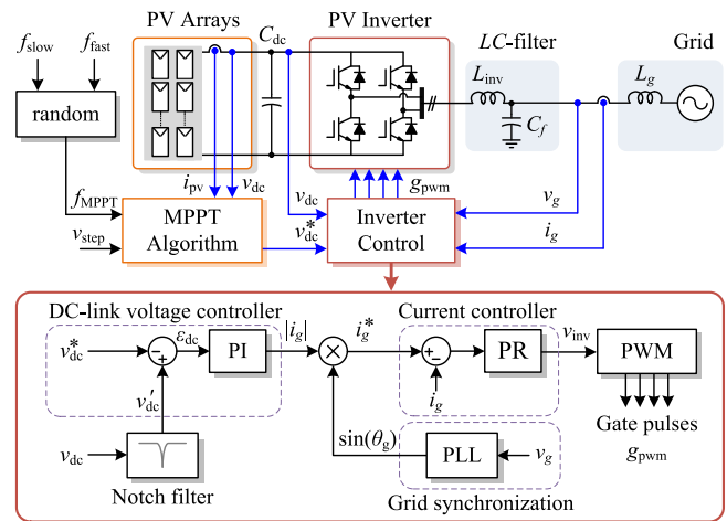
Fig. 1. System diagram and control structure of single-stage single-phase PV inverter (PI: proportional integral, PR: proportional resonant, PWM: pulswidth modulation, PLL: phase-locked loop).
