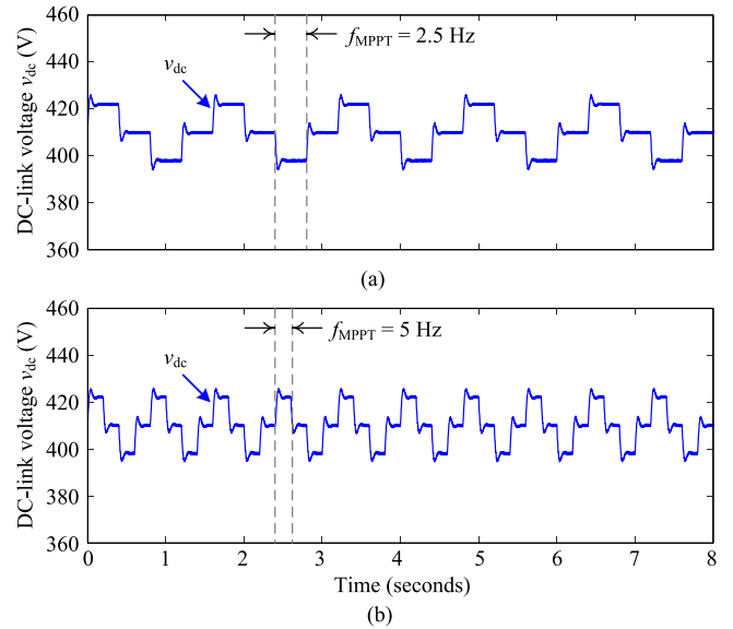
Fig. 2. Experimental waveforms of the dc-link voltage v_{dc} of the PV inverter operated at 10% of the rated power (i.e., 0.3 kW) with the MPPT sampling rate of (a) f_{MPPT} = 2.5 \text{ Hz} and (b) f_{MPPT} = 5 \text{ Hz} .
