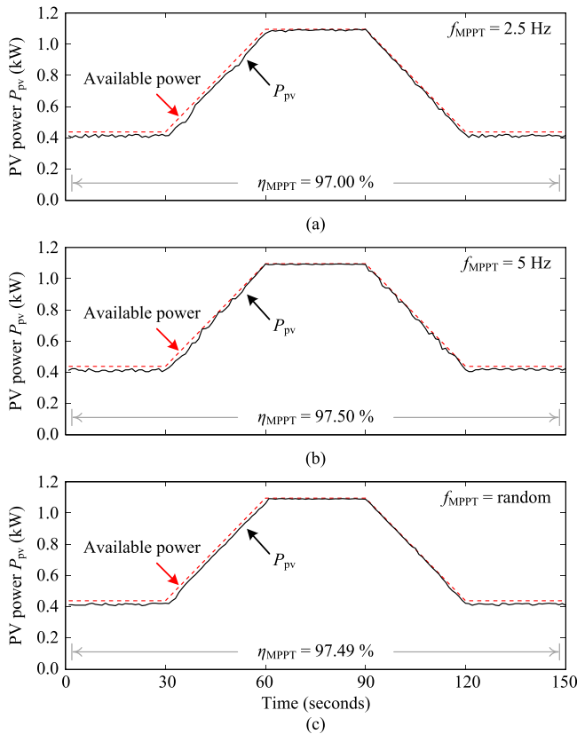
Fig. 7. Measured PV power extraction of the PV inverter under the trapezoidal solar irradiance condition with the MPPT sampling rate of (a) f_{\text{MPPT}} = 2.5 Hz, (b) f_{\text{MPPT}} = 5 Hz, and (c) f_{\text{MPPT}} = \text{random} .
