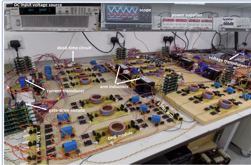
Fig. 16. Hardware view of the experimental prototype.
