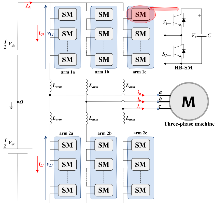
Fig. 1. Circuit diagram of a conventional MMC topology feeding a three-phase induction machine.
