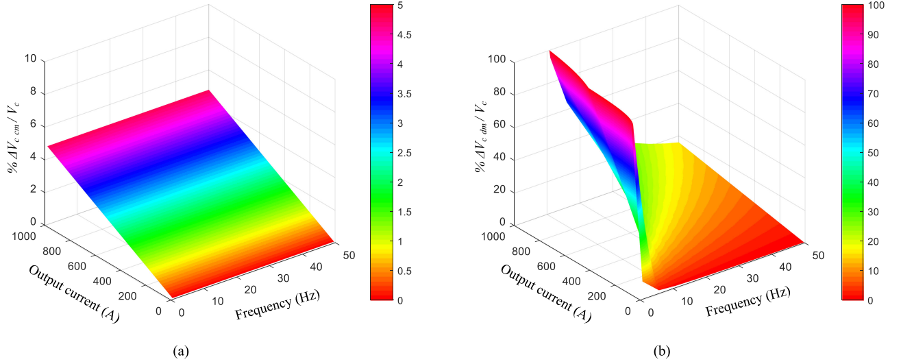
Fig. 3. Relation curves of capacitor voltage-ripple at constant M/\omega versus operating frequency and output current for (a) CM component and (b) DM component. ( C = 3 mF, V_c = 2.5 kV, and \varphi = 35^\circ ).
