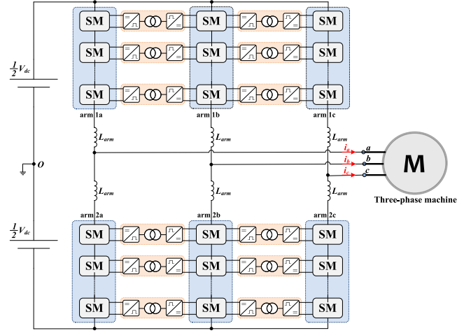
Fig. 10. Alternative structure of the proposed MMC configuration with reduced number of DHB modules.
