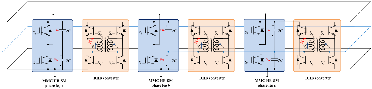
Fig. 7. DHB-based power decoupling chain for three MMC adjacent-arm HB-SMs.
