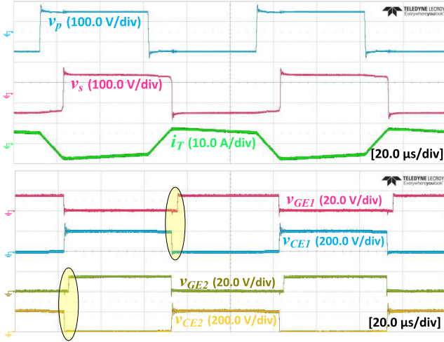
Fig. 22. DHB converter switching waveforms at rated parameters.
