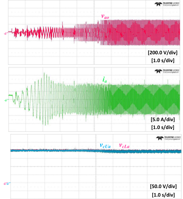
Fig. 23. Dynamic performance of the proposed drive system when starting an induction motor from standstill to the rated speed at rated torque.
