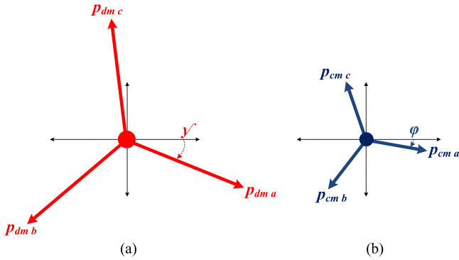
Fig. 5. Phasor representation for MMC arm power components in the (a) fundamental-frequency domain and (b) second-order frequency domain.
