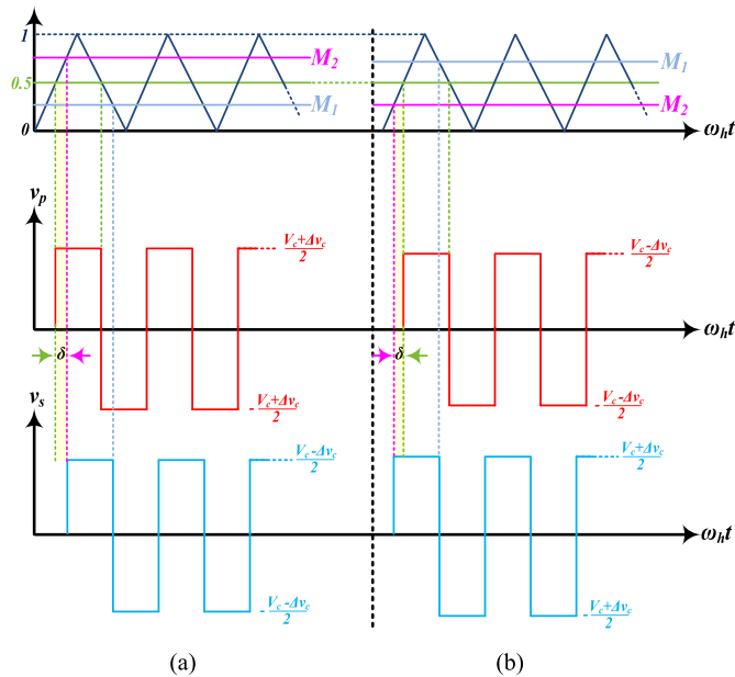
Fig. 8. Sketch of the phase-shift PWM of a DHB converter for bidirectional power transfer. (a) Positive phase-shift angle. (b) Negative phase-shift angle.
