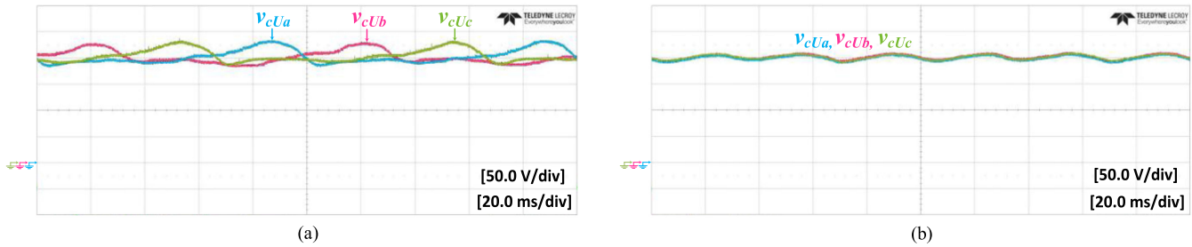
Fig. 19. Capacitor voltage fluctuation at 10 Hz when the DHB scheme is (a) deactivated and (b) activated.
