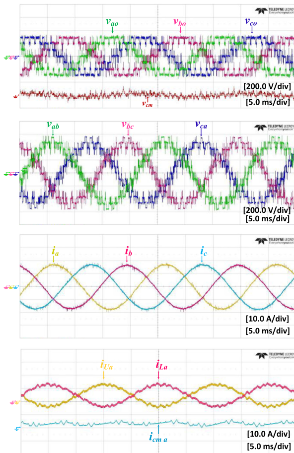
Fig. 17. Experimental waveforms of the MMC system at rated parameters.
