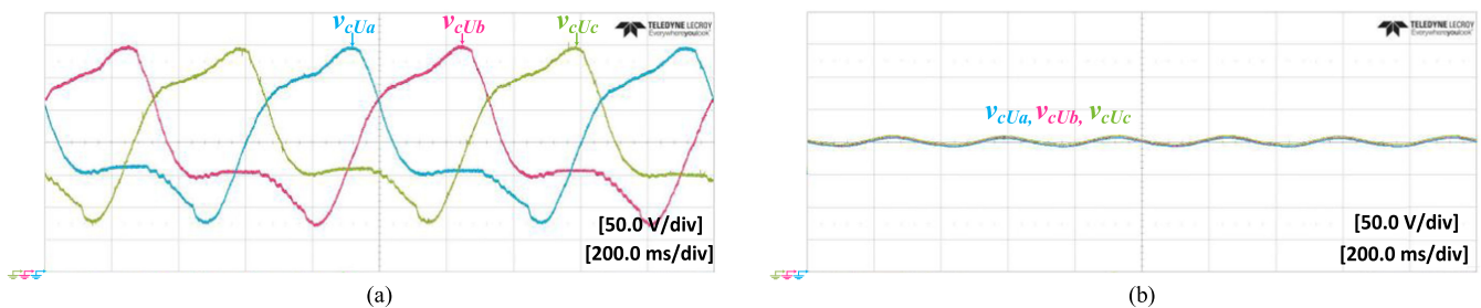
Fig. 21. Capacitor voltage fluctuation at 1 Hz when the DHB scheme is (a) deactivated and (b) activated.
