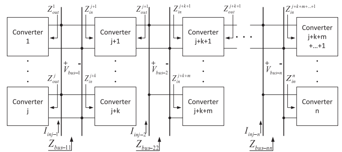
Fig. 1. Conceptual multibus system showing multiple interconnections [3].
