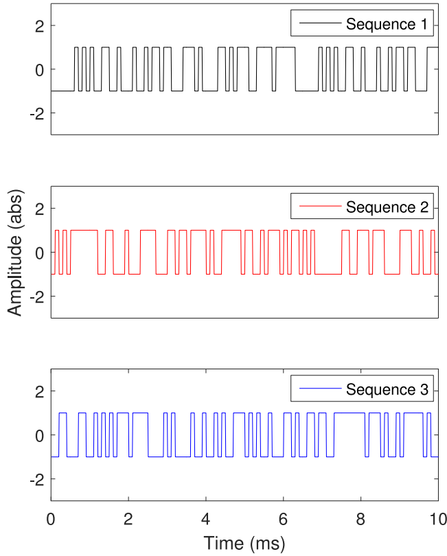
Fig. 3. Three orthogonal sequences in time domain.
