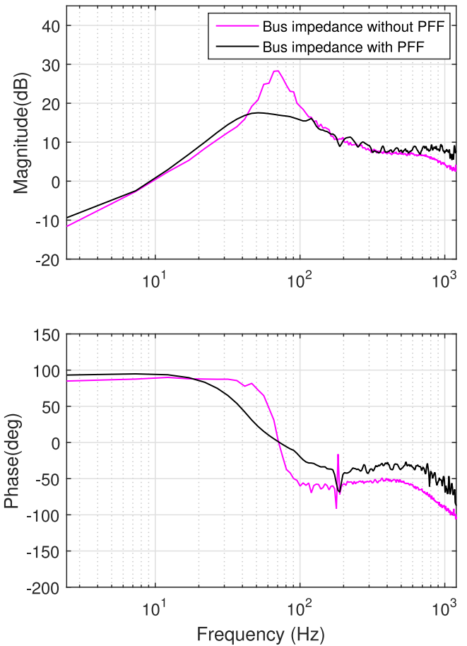
Fig. 15. Bus impedance with and without positive feedforward controller.
