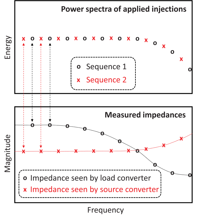
Fig. 7. Obtaining simultaneously several impedances.
