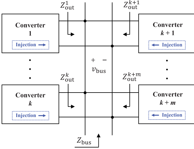
Fig. 2. Multiconverter system.
