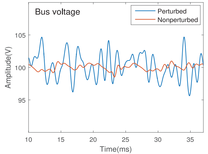
Fig. 13. Sample of perturbed and nonperturbed bus voltage.
