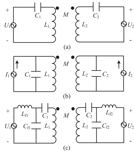
Fig. 1. Topologies of a WPT system. (a) SS. (b) PP. (c) LCC-LCC.
