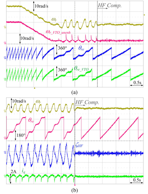
Fig. 12. Low speed behavior when the drive is equipped with a 3 BPP position sensing system and the VTO is tuned for a 20 Hz bandwidth. (a) Transient from 20 to 3 rad/s. (b) Operation for reference speed set to 3 rad/s.
