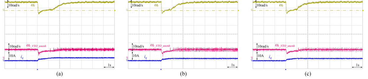
Fig. 18. Disturbance response transient following a 0.4 p.u. step load at 10 rad/s, with signal injection. (a) 3 BPP. (b) 2 BPP. (c) 1 BPP.
