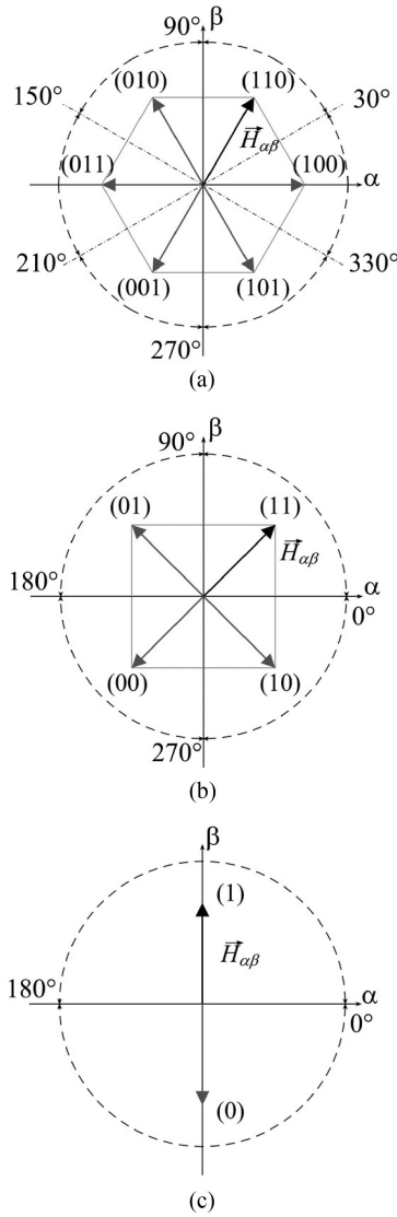
Fig. 1. Quantized rotating position vector \mathbf{H}_{\alpha\beta} loci for low-resolution position sensing systems [14]. (a) 3 BPP. (b) 2 BPP. (c) 1 BPP.
