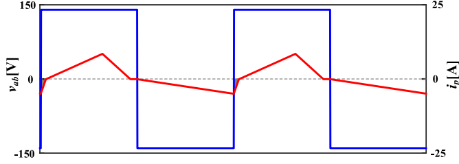
Fig. 8. Waveforms of v_{ab} and i_p in the FB-SC converter with V_i = 140 V and P_o = 500 W.
