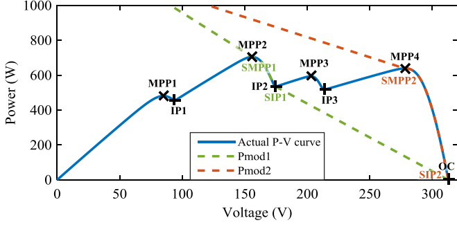
Fig. 4. Modification of multipeak P - V curves.
