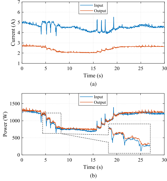
Fig. 14. Oscillograms of the input and the output. (a) Current. (b) Power of the converter.
