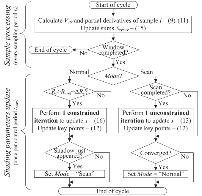
Fig. 9. Flowchart of the MPPs estimation algorithm. The upper part is executed every sampling period t_s = 50 \mu s , whereas the lower part once per control period t_{conv} = 20 ms.
