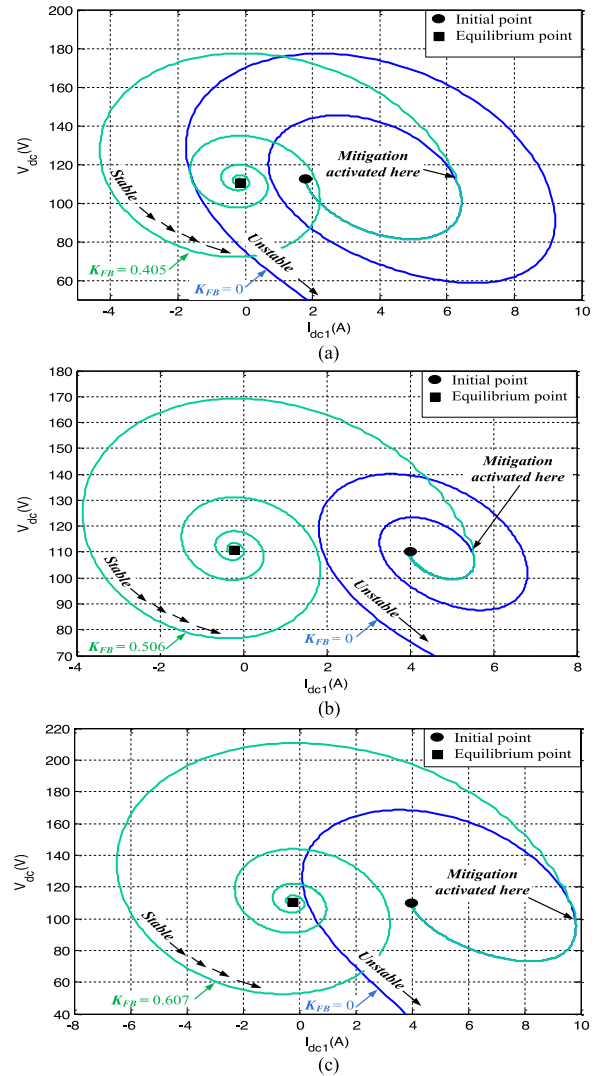
Fig. 9. Phase-plane plots of the system with the proposed adaptive stabilization. (a) P_{CPL} = 400 W. (b) P_{CPL} = 500 W. (c) P_{CPL} = 600 W.
