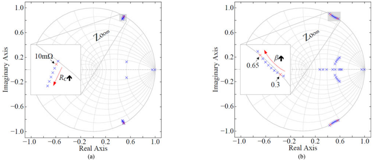
Fig. 10. Damping of the critically stable point at L_g = L_{g,crit} = 360 \mu\text{H} . (a) Effect of the capacitor ESR. (b) Effect of the capacitance deviation with R_C = 10 \text{ m}\Omega .
