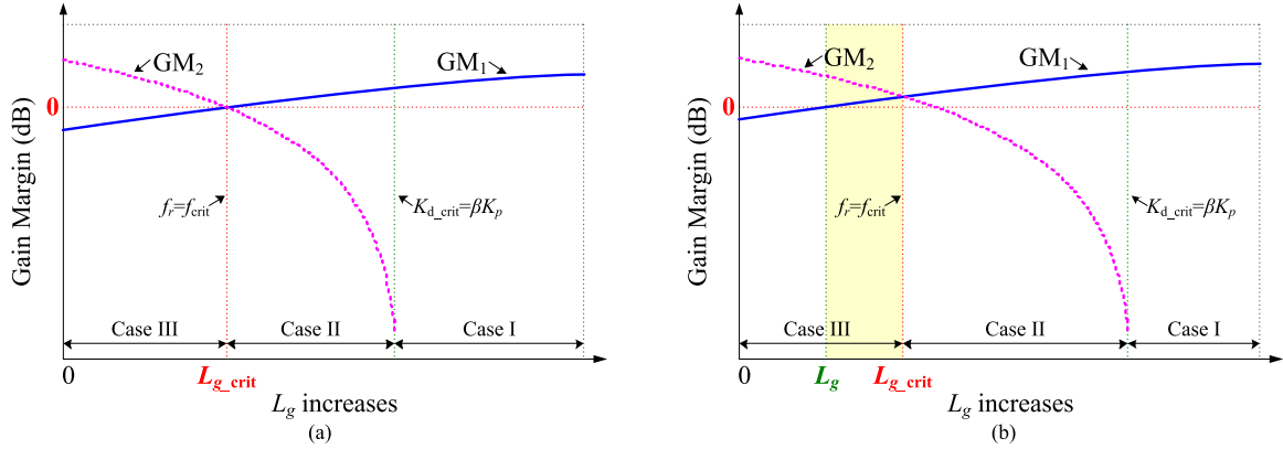
Fig. 5. Curves of GM_1 and GM_2 with the increase of L_g . (a) \beta = L_1/(L_1 + L_2 + L_{g,crit}) . (b) \beta = L_1/(L_1 + L_2 + L_g) .
