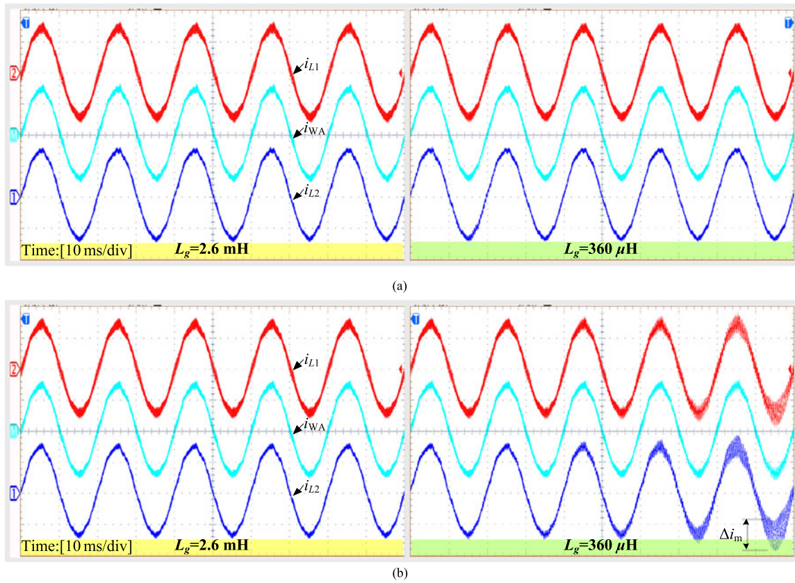
Fig. 12. Experimental results at full load under the grid impedance variation. (a) \beta = L_1 / (L_1 + L_2 + L_{g,crit}) = 0.5 . (b) \beta = L_1 / (L_1 + L_2 + L_g) = 0.8 (initialized with L_g = 0 ). Current waveform scales: 30 A/div.
