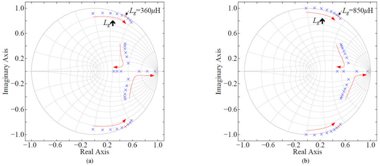
Fig. 9. Grid current closed-loop pole maps with L_g varying up to 2.6 mH. (a) \beta = L_1/(L_1 + L_2 + L_{g,crit}) = 0.5 . (b) \beta = L_1/(L_1 + L_2 + L_g) = 0.8 (initialized with L_g = 0 ).
