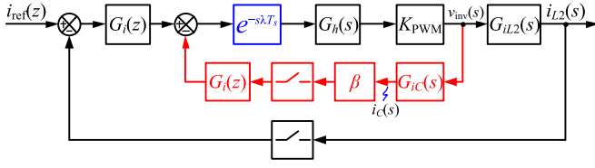
Fig. 4. Equivalent transformation of the block diagram of the weighted average current control.
