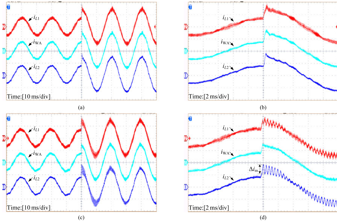
Fig. 11. Experimental results when the current reference steps from half to full loads at L_g = 0 . (a) \beta = L_1 / (L_1 + L_2 + L_{g,crit}) = 0.5 . (b) Zoom of (a). (c) \beta = L_1 / (L_1 + L_2 + L_g) = 0.8 (initialized with L_g = 0 ). (d) Zoom of (c). Current waveform scales: 30 A/div.
