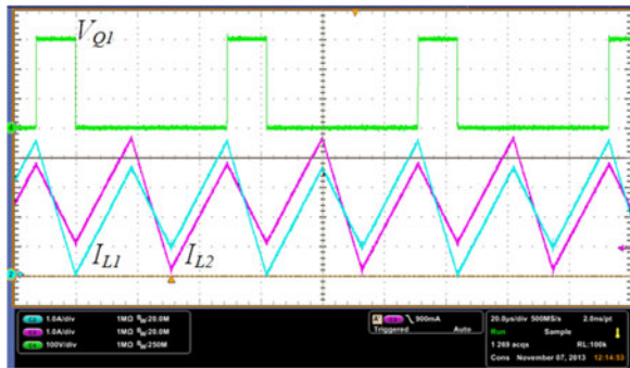
Fig. 10. Experimental waveforms of CCM. The Q1 voltage (green) is 100 V/div, whereas the phase 1 current (blue) and phase 2 current (purple) are 1 A/div each [10].
