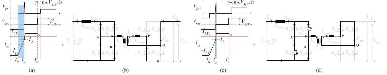
Fig. 7. Equivalent circuit diagrams for Mode III operation in DPSM: (a) and (b) Interval I ( t_0-t_\varphi ) same as Mode II; (c) and (d) voltage spike due to the turn OFF of S_2 and S_3 .
