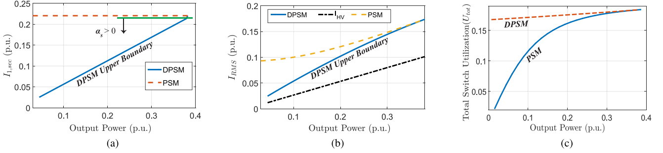
Fig. 9. (a) Plot of I_{1,sec} through the series inductor versus output power for DPSM (solid line) and PSM (dashed line); (b) plot of I_{RMS,sec} for DPSM (solid line) and PSM (dashed line) and the HV current ( I_{HV} ) for different output powers. The plot for DPSM is for the upper boundary condition given in (21). At around 0.37 p.u. output power, \alpha_s = 0 and DPSM reduces to PSM. (c) Plot of total LV switch utilization versus output power for DPSM (dashed line) and PSM (solid lines).
