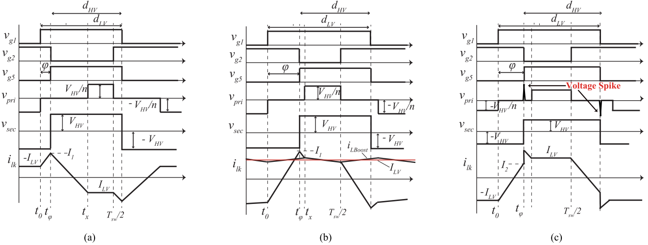
Fig. 2. Basic operating waveforms for PSM with fixed HV duty ( d_{HV} = 0.5 ) and LV duty d_{LV} = (0.5 + \varphi) : (a) Mode I: 0 < \varphi \leq x/2 and P < 0 , (b) Mode II: x/2 < \varphi < \varphi_{max} and 0 < P \leq P_{max} , (c) Mode III: \varphi_{max} < \varphi < 0.5 and P > P_{max} .
