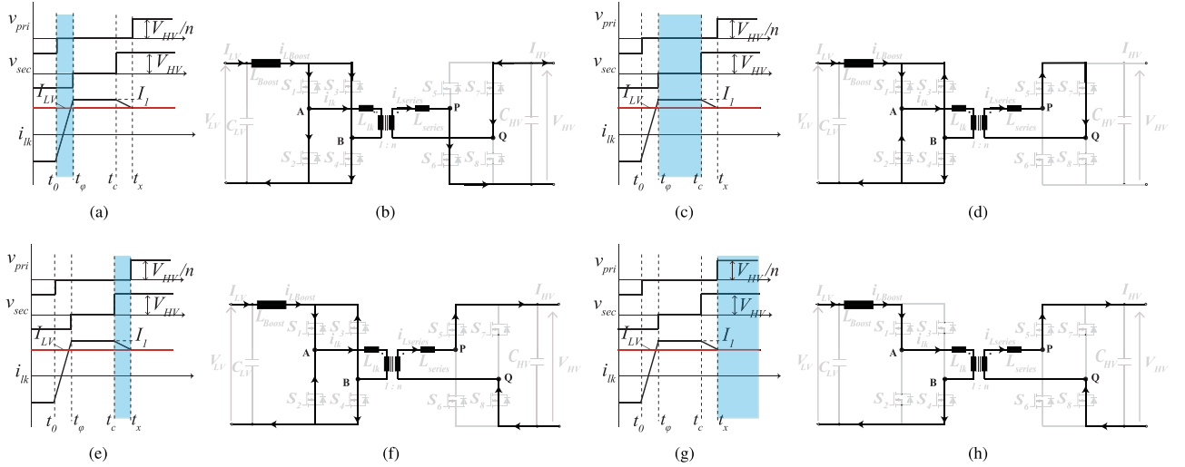
Fig. 6. Equivalent circuit diagrams for Mode II operation in DPSM: (a) and (b) Interval I ( t_0-t_\varphi ); (c) and (d) Interval II ( t_\varphi-t_c ) with t_c = (t_\varphi+t_{\alpha_s}) ; (e) and (f) Interval III ( t_c-t_x ); (g) and (h) Interval IV ( t_x-T_{sw}/2 ).
