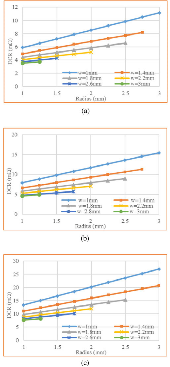
Fig. 6. DCR versus radius with coil width as a parameter. (a) N = 4.5 . (b) N = 5.5 . (c) N = 6.5 .
