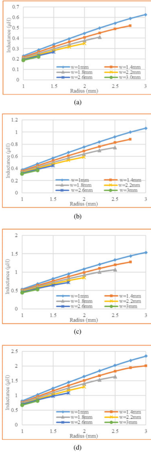
Fig. 5. Inductance versus radius with coil width as a parameter. (a) N = 3.5 . (b) N = 4.5 . (c) N = 5.5 . (d) N = 6.5 .
