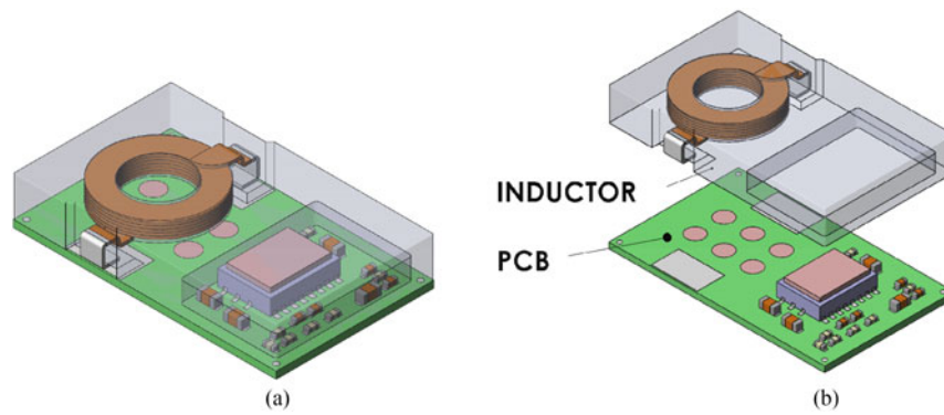
Fig. 3. Proposed magnetic packaging. (a) Magnetic packaging power module. (b) Internal structure.
