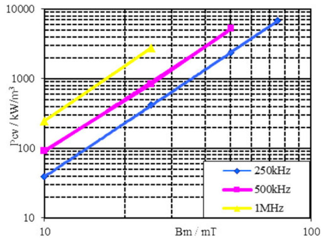
Fig. 13. Loss characteristics of the magnetic material.
