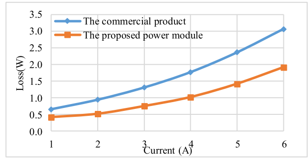
Fig. 21. Loss of the two power modules.
