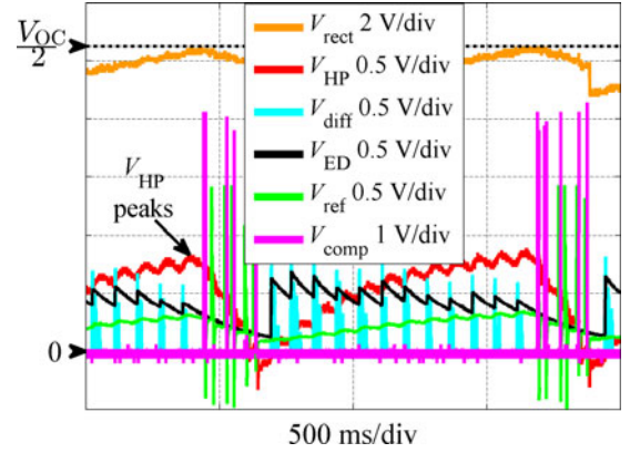
Fig. 5. Measured V_{rect} , V_{HP} , V_{diff} , V_{ED} , V_{ref} , and V_{comp} to show the operation of the implemented analog control circuit in enabling the buck converter for power transfer when the PEH is subjected to a peak-to-peak strain loading of 300 \mu\epsilon at 6 Hz.
