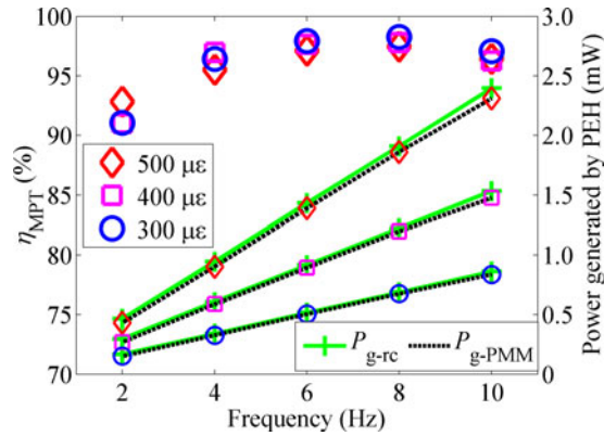
Fig. 7. \eta_{\text{MPT}} of the proposed circuit obtained by comparing the power generated by the PEH using circuit CFG 1, P_{\text{g-PMM}} (dashed) with the power generated by the PEH using circuit CFG 2, P_{\text{g-rc}} (solid) at different frequencies and strain levels of 300 \mu\epsilon (○), 400 \mu\epsilon (□), and 500 \mu\epsilon (◇).
