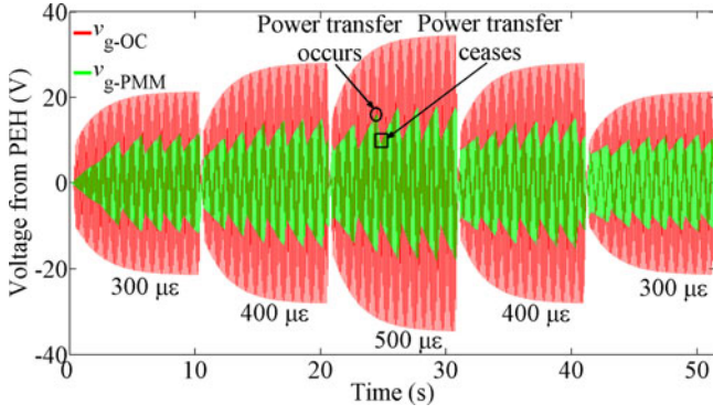
Fig. 9. Measured v_{g-OC} (higher amplitude) and v_{g-PMM} generated by the PEH when it is open-circuited and connected to the power management module, respectively, in a sweep test. Peak voltage of v_{g-PMM} is around V_{OC}/2 when power transfer occurs, as pointed at one of the occurrences circled in the figure.
