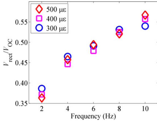
Fig. 6. Ratio of V_{\text{rect}} to V_{\text{OC}} at different strain levels and frequencies showing that energy can be harvested away from V_{\text{OC}}/2 .
