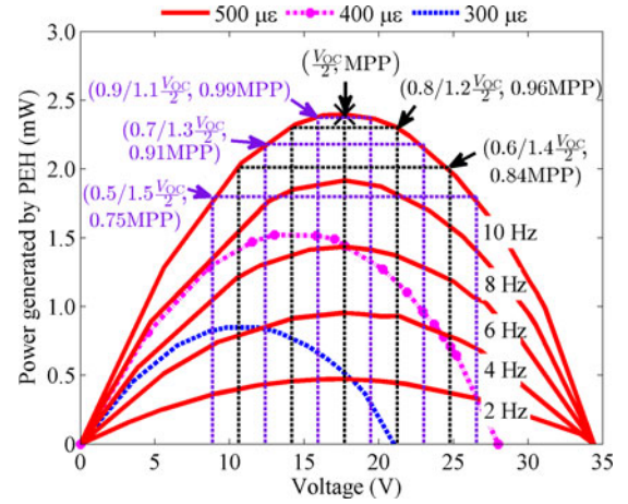
Fig. 8. Matter of accuracy in finding MPP based on V_{\text{OC}}/2 method by using strain loading of 500 \mu\epsilon (solid) at different frequencies as example. Power curves for strain loadings of 300 \mu\epsilon (dashed) and 400 \mu\epsilon (dashed-dotted) at 10 Hz are also plotted to show that the method works for different V_{\text{OC}} .
