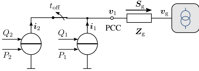
Fig. 4. Exemplary system of two grid-connected DG units.
