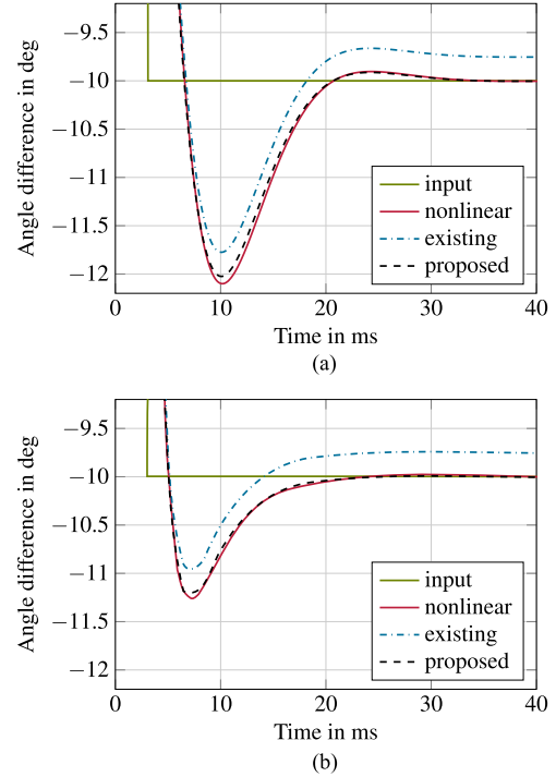
Fig. 5. Comparison of SRF-PLL models as a result of a fault, parameterized with (a) \zeta_{cl} = 0.707 , \omega_{cl} = 2\pi 50 \frac{\text{rad}}{\text{s}} and (b) \zeta_{cl} = 0.8 , \omega_{cl} = 2\pi 100 \frac{\text{rad}}{\text{s}} .
