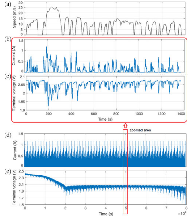
Fig. 14. Li-S cell discharge test based on UDDS drive cycle. (a) UDDS speed profile. (b) Li-S cell current profile based on one UDDS cycle. (c) Terminal voltage of a Li-S cell during one UDDS cycle. (d) Repeating UDDS current profile. (e) Li-S cell's terminal voltage during UDDS test.
