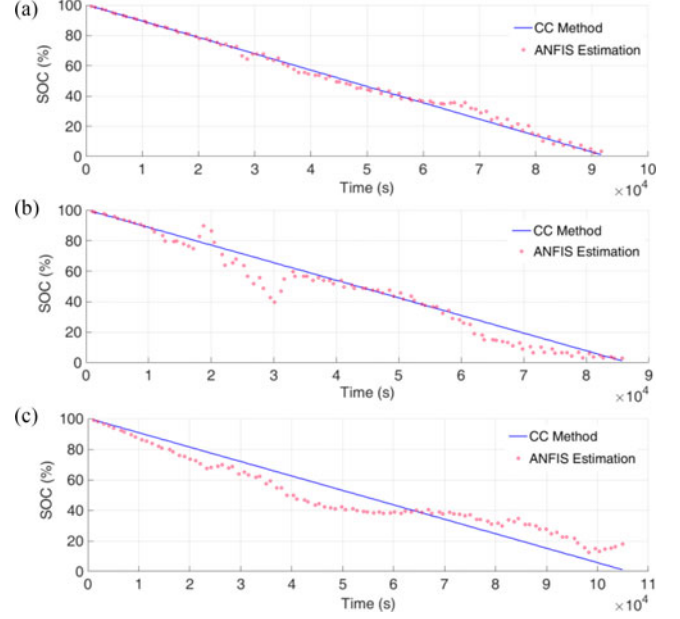
Fig. 10. Actual SOC and ANFIS estimations using V_{OC} and R_O . (a) Training data. (b) Test data 1. (c) Test data 2.
