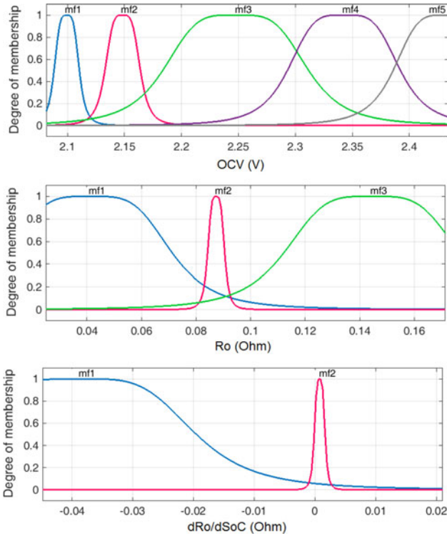
Fig. 12. ANFIS inputs MFs after training.
