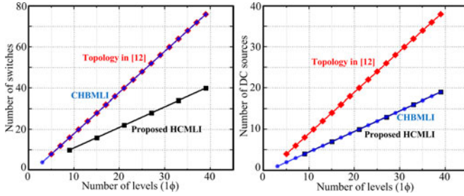
Fig. 5. Number of switches and dc sources as a function of the number of voltage levels for single-phase inverter.
