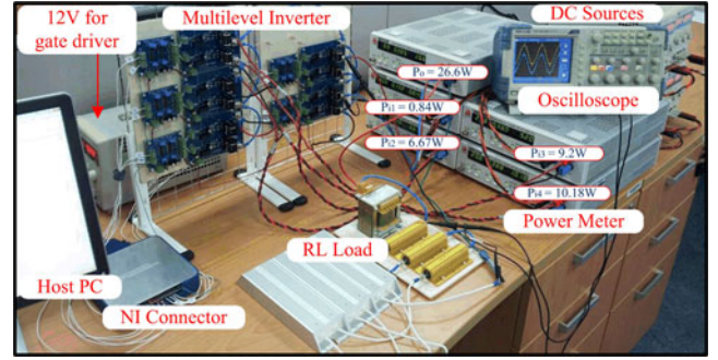
Fig. 6. Experimental prototype of the proposed MLI topology.
