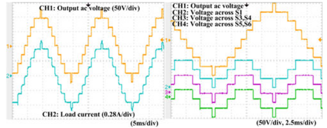
Fig. 7. Experimental waveforms with four 30V dc supplies ( R = 180 \Omega , L = 11 \text{ mH} ). (a) Output voltage and load current. (b) Output voltage and voltages across switches in the proposed submodule.
