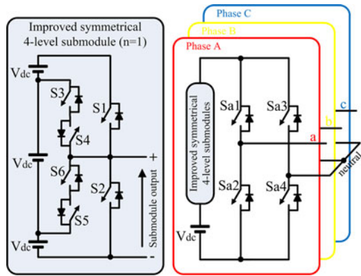
Fig. 2. Circuit diagram of the proposed MLI topology.
