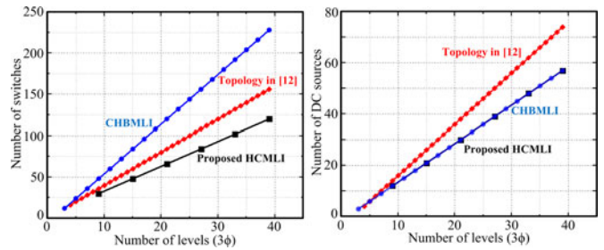
Fig. 3. Number of switches and dc sources as a function of the number of voltage levels for a three-phase inverter.
