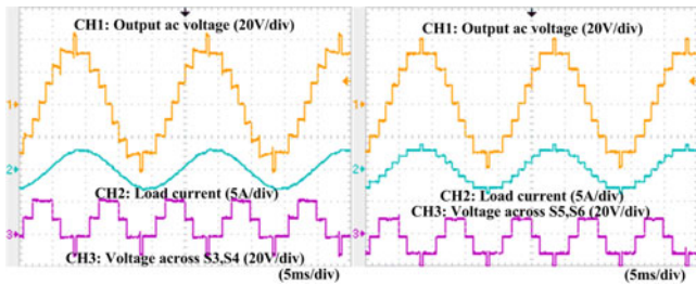
Fig. 8. Experimental waveforms with four 12 V battery sources. (a) R = 10 \Omega , L = 11 \text{ mH} . (b) R = 10 \Omega .
