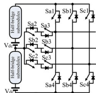
Fig. 1. Optimized MLI topology presented in [12].
