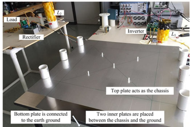
Fig. 6. Prototype of a downsized two-plate CPT system with a ground-side plate.
