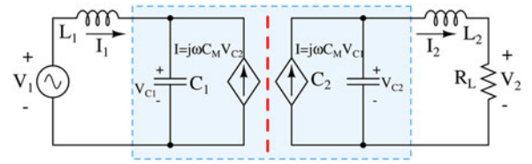
Fig. 4. Simplified circuit topology of a two-plate CPT system.
