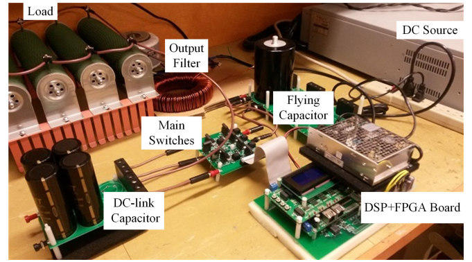
Fig. 19. Experimental prototype.
