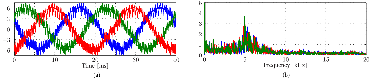
Fig. 15. Experimental results of the ac side of the qZSI with MPC and a 1T_s prediction horizon length. The sampling interval is T_s = 25 \mu\text{s} and \lambda_u = 0.42 . The switching frequency is f_{sw} \approx 5 \text{ kHz} and the output current THD I_{o, \text{THD}} = 17.05\% . (a) Three-phase output current i_o (solid lines) and their references (dash-dotted lines) in [A]. (b) Output current spectrum (%).
