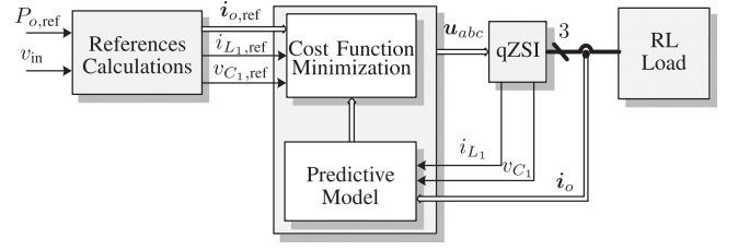
Fig. 4. Direct MPC with reference tracking for the qZSI.
