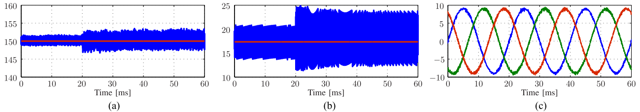
Fig. 12. Simulation results for MPC and a 5T_s prediction horizon length when L_1 and L_2 of the qZS network are reduced by 50%. (a) Capacitor voltage v_{C_1} and its reference in [V]. (b) Inductor current i_{L_1} and its reference in [A]. (c) Three-phase output current i_o (solid lines) and their references (dash-dotted lines) in [A].
