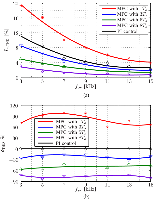
Fig. 8. Tradeoff between the output current THD I_{o,THD} and the switching frequency f_{sw} for the PI-based controller and the MPC with prediction horizon length of 1T_s , 3T_s , 5T_s , and 8T_s . (a) Current THD and switching frequency. (b) Relative current THD and switching frequency.
