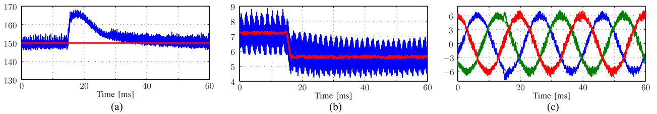
Fig. 24. Experimental results for a step change in the input dc voltage with a PI-based controller. (a) Capacitor voltage v_{C1} and its reference in [V]. (b) Inductor current i_{L1} and its reference in [A]. (c) Three-phase output current i_o (solid lines) and their references (dash-dotted lines) in [A].
