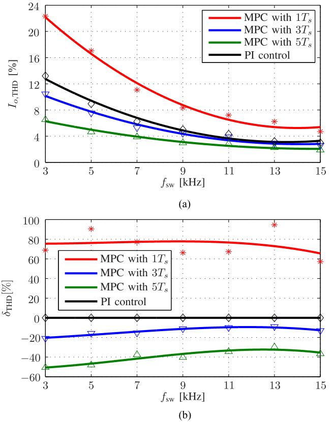
Fig. 20. Tradeoff between the output current THD I_{o,THD} and the switching frequency f_{sw} for the PI-based controller and the MPC with prediction horizon length of 1T_s , 3T_s , and 5T_s . (a) Current THD and switching frequency. (b) Relative current THD and switching frequency.
