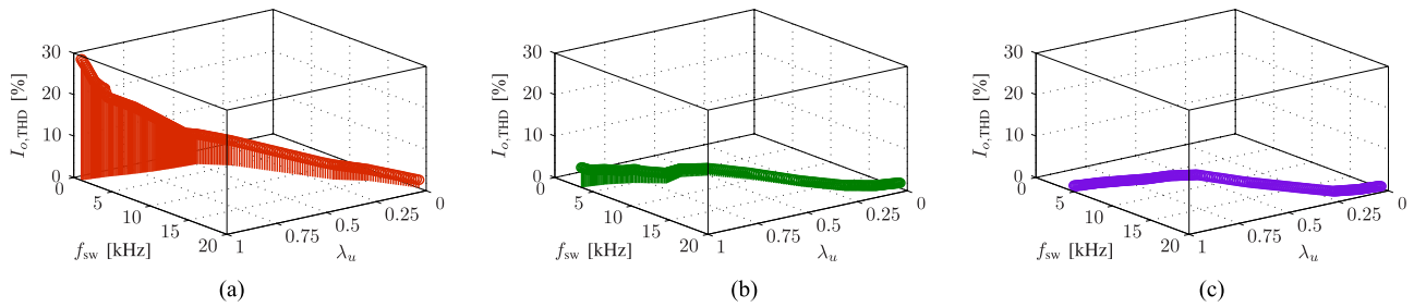
Fig. 7. Effect of the weighting factor ( \lambda_u ) on the switching frequency and the output current THD for the MPC with different prediction horizons ( 1T_s , 5T_s , and 8T_s ). (a) MPC with 1T_s . (b) MPC with 5T_s . (c) MPC with 8T_s .
