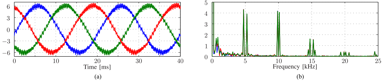
Fig. 19. Experimental results of the ac side of the qZSI with PI-based control. The switching frequency is f_{sw} = 5 kHz and the output current THD I_{o,THD} = 8.95\% . (a) Three-phase output current i_o (solid lines) and their references (dash-dotted lines) in [A]. (b) Output current spectrum (%).
