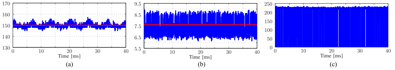
Fig. 14. Experimental results of the dc side of the qZSI with MPC and an 1T_s prediction horizon length. The sampling interval is T_s = 25 \mu\text{s} and \lambda_u = 0.42 . The switching frequency is f_{sw} \approx 5 \text{ kHz} . (a) Capacitor voltage v_{C1} and its reference in [V]. (b) Inductor current i_{L1} and its reference in [A]. (c) DC-link voltage v_{dc} in [V].
