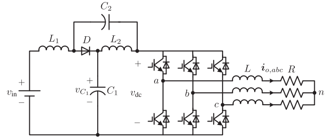
Fig. 1. Topology of the qZSI.
