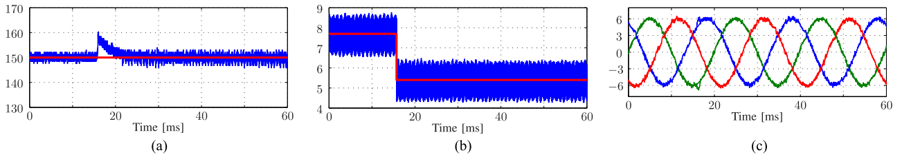
Fig. 23. Experimental results for a step change in the input dc voltage with MPC and a 5T_s prediction horizon length. (a) Capacitor voltage v_{C1} and its reference in [V]. (b) Inductor current i_{L1} and its reference in [A]. (c) Three-phase output current i_o (solid lines) and their references (dash-dotted lines) in [A].
