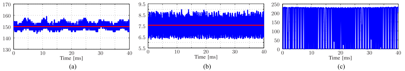
Fig. 16. Experimental results of the dc side of the qZSI with MPC and a 5T_s prediction horizon length. The sampling interval is T_s = 25 \mu\text{s} and \lambda_u = 0.75 . The switching frequency is f_{sw} \approx 5 \text{ kHz} . (a) Capacitor voltage v_{C1} and its reference in [V]. (b) Inductor current i_{L1} and its reference in [A]. (c) DC-link voltage v_{dc} in [V].
