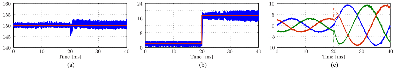
Fig. 10. Simulation results for a step change in the output current reference with MPC and a 5T_s prediction horizon length. (a) Capacitor voltage v_{C_1} and its reference in [V]. (b) Inductor current i_{L_1} and its reference in [A]. (c) Three-phase output current i_o (solid lines) and their references (dash-dotted lines) in [A].
