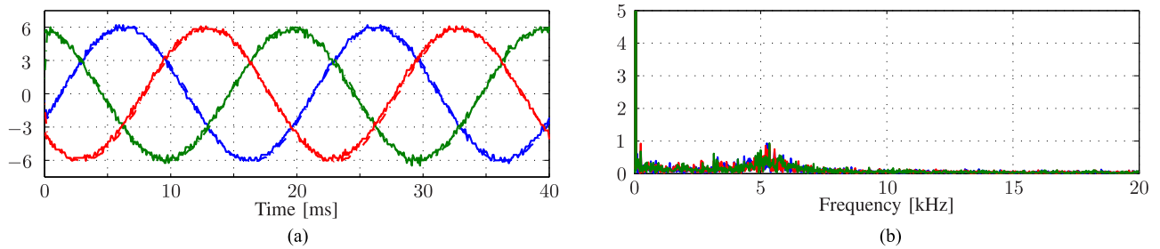
Fig. 17. Experimental results of the ac side of the qZSI with MPC and a 5T_s prediction horizon length. The sampling interval is T_s = 25 \mu\text{s} and \lambda_u = 0.75 . The switching frequency is f_{sw} \approx 5 \text{ kHz} and the output current THD I_{o, \text{THD}} = 4.65\% . (a) Three-phase output current i_o (solid lines) and their references (dash-dotted lines) in [A]. (b) Output current spectrum (%).
