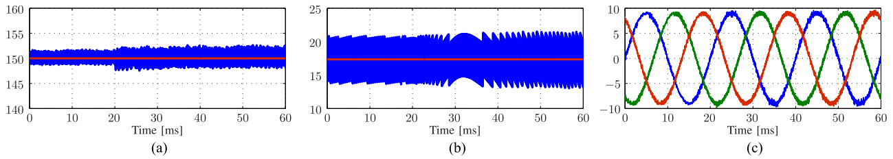
Fig. 11. Simulation results for MPC and a 5T_s prediction horizon length when R of the RL load is reduced by 50%. (a) Capacitor voltage v_{C_1} and its reference in [V]. (b) Inductor current i_{L_1} and its reference in [A]. (c) Three-phase output current i_o (solid lines) and their references (dash-dotted lines) in [A].
