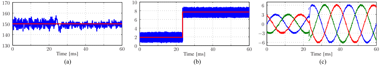
Fig. 21. Experimental results for a step change in the output current reference with MPC and a 5T_s prediction horizon length. (a) Capacitor voltage v_{C1} and its reference in [V]. (b) Inductor current i_{L1} and its reference in [A]. (c) Three-phase output current i_o (solid lines) and their references (dash-dotted lines) in [A].
