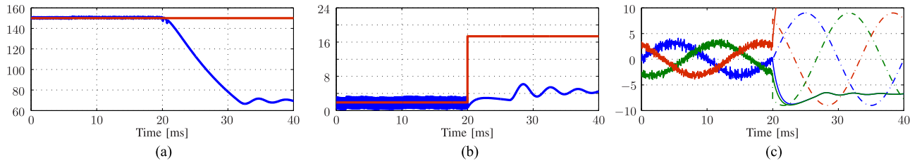
Fig. 9. Simulation results for a step change in the output current reference with MPC and a 1T_s prediction horizon length. (a) Capacitor voltage v_{C_1} and its reference in [V]. (b) Inductor current i_{L_1} and its reference in [A]. (c) Three-phase output current i_o (solid lines) and their references (dash-dotted lines) in [A].
