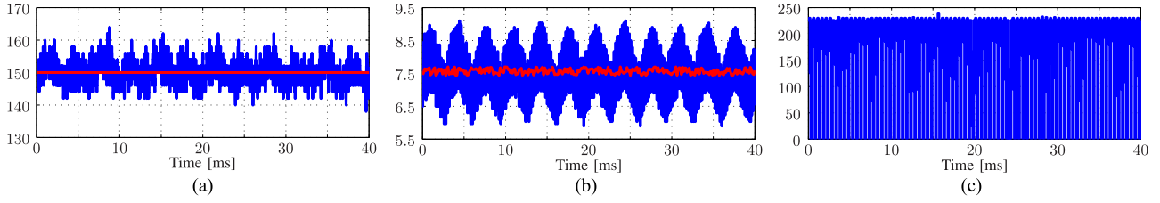
Fig. 18. Experimental results of the dc side of the qZSI with PI-based control. The switching frequency is f_{sw} = 5 kHz. (a) Capacitor voltage v_{C1} and its reference in [V]. (b) Inductor current i_{L1} and its reference in [A]. (c) DC-link voltage v_{dc} in [V].
