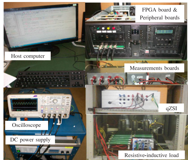
Fig. 13. System set-up in the laboratory.
