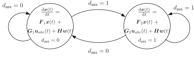
Fig. 3. qZSI presented as a continuous-time automaton.
