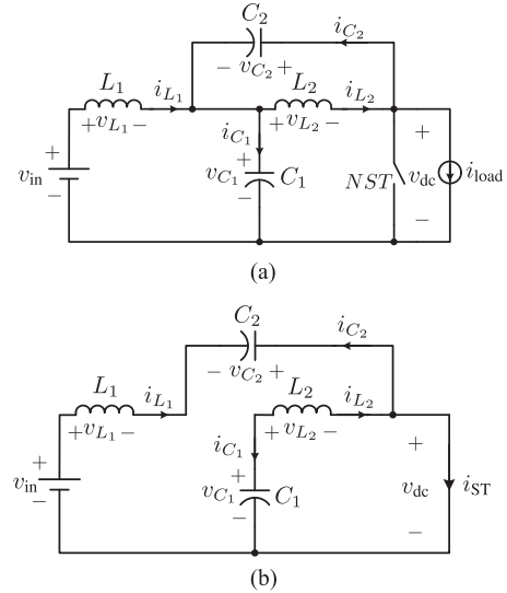
Fig. 2. Operation states of the qZSI. (a) Non-shoot-through state. (b) Shoot-through state
