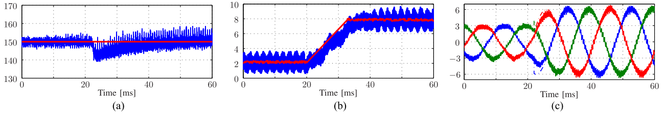
Fig. 22. Experimental results for a step change in the output current reference with a PI-based controller. (a) Capacitor voltage v_{C1} and its reference in [V]. (b) Inductor current i_{L1} and its reference in [A]. (c) Three-phase output current i_o (solid lines) and their references (dash-dotted lines) in [A].
