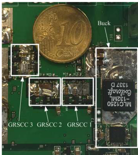
Fig. 12. Photograph of the hybrid-VRM power stage, including the buck converter and three interleaved GRSCCs.
