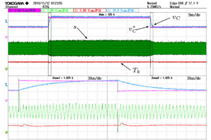
Fig. 15. Regulation: v_C^* variation from 12 to 24 V and vice versa, with R = 4 \Omega . v_C : blue; s : green; v_C^* : magenta; T_k : red.
