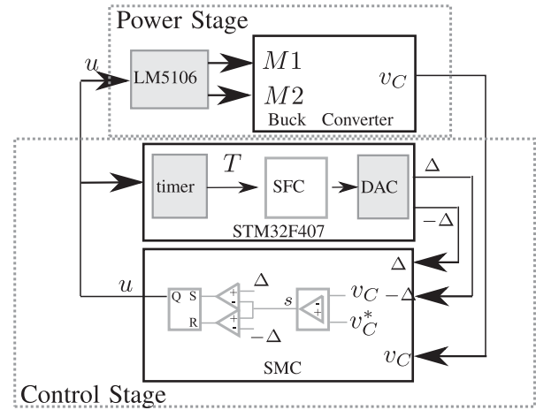
Fig. 11. Implementation details: the SMC with a variable hysteresis comparator is implemented using analogue circuitry, while the SFC is implemented using a DSP STM32F407.
