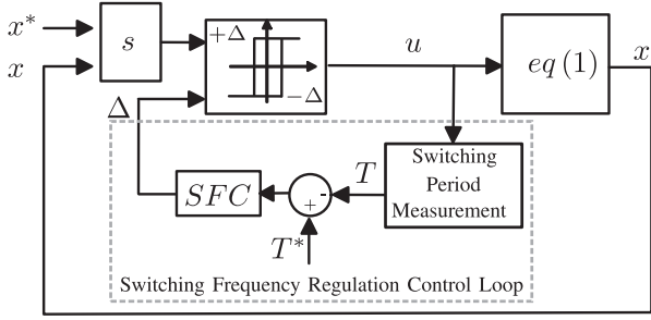
Fig. 3. Overall controller architecture.
