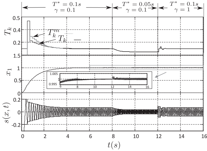
Fig. 6. Regulation: Performance of the SFC for different values of \gamma and T^* .
