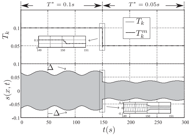
Fig. 8. Tracking: evolution of T_k and s when T^* is changed from 0.1 to 0.05 s.
