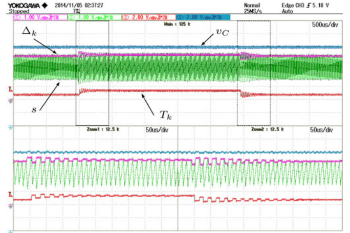
Fig. 16. Regulation: underdamped responses for \gamma = 200 000 with R = 4 \Omega and a T^* variation from 12.5 \mu s 14 \mu s. v_C : blue; s : green; |\Delta_k| : magenta; T_k : red.
