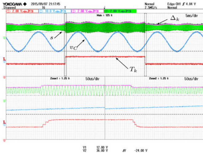
Fig. 18. Tracking: T^* variation from 9\mu\text{s} to 14\mu\text{s} . v_C : blue; s : green; |\Delta_k| : magenta; T_k : red.
