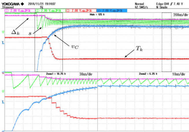
Fig. 14. Regulation: start-up for v_C^* = 12 V with R = 2 \Omega and \Delta_0 higher than the steady-state value. v_C : blue; s : green; |\Delta_k| : magenta; T_k : red.
