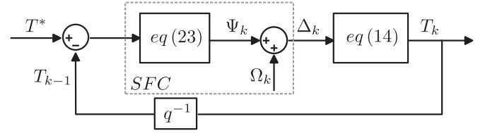
Fig. 5. Switching frequency regulation control loop with feedforward action.
