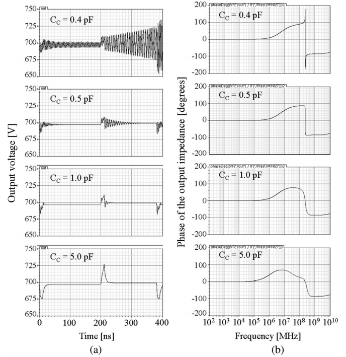
Fig. 13. Output response of a distributed power delivery system with different compensation ( C_C = 0.4 pF, C_C = 0.5 pF, C_C = 1 pF, and C_C = 5 pF), showing the correlation between the (a) transient response, and (b) phase of the output impedance.
