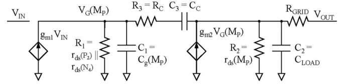
Fig. 5. Small signal linear model of LDO.
