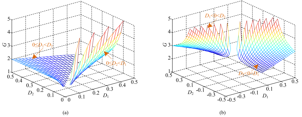
Fig. 7. Characterization of current impact. (a) Constant power flow. (b) Different power flows.
