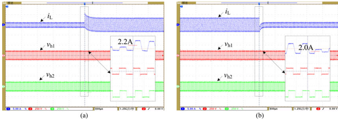
Fig. 10. Transient experimental waveforms under the SPS updating strategy with constant flow. (a) Increases in power. (b) Decreases in power.
