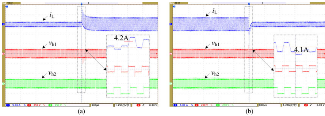
Fig. 11. Transient experimental waveforms under the SPS updating strategy with different flows. (a) From reverse to forward power flow. (b) From forward to reverse power flow.
