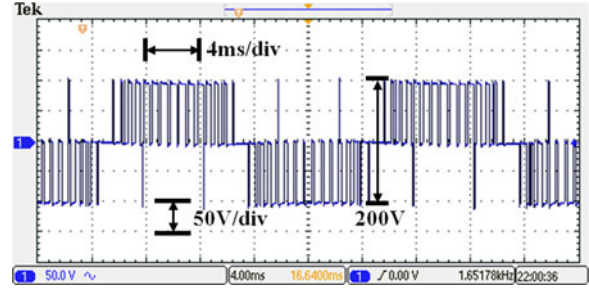
Fig. 10. Line voltage generated by switching angles II in Table V.
