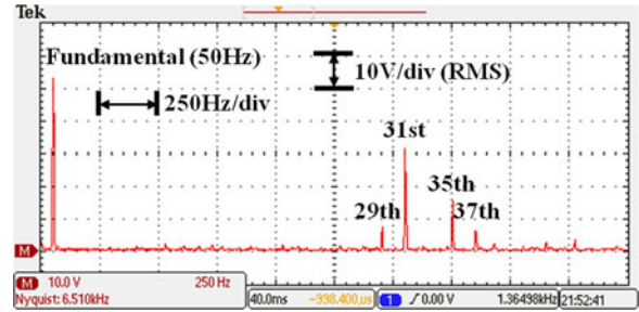
Fig. 11. FFT results of the line voltage shown in Fig. 10.
