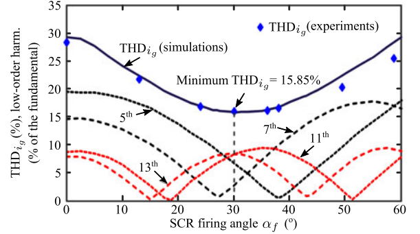
Fig. 6. THD_{i_g} and low-order harmonics of the grid current in the multidrive system with the phase-shifted current control.
