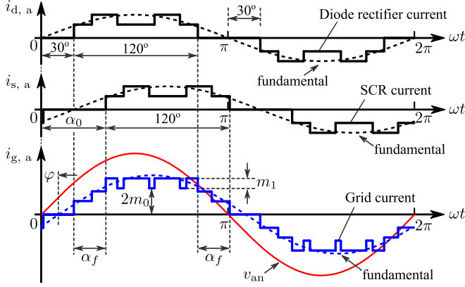
Fig. 5. Typical waveforms of the phase-A currents in a multidrive system (see Fig. 1) with the proposed modulation scheme and the phase-shifted control, where the current shapes follow the modulation pattern in Fig. 4.
