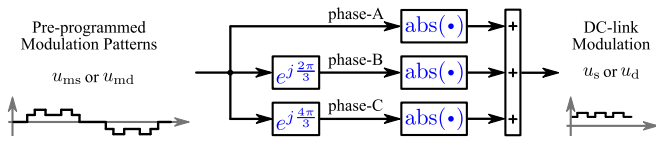
Fig. 3. Synthesis process of the proposed dc-link current modulation scheme for the drive systems shown in Fig. 1, where u_s and u_d are the synthesized dc-link current modulation signals.
