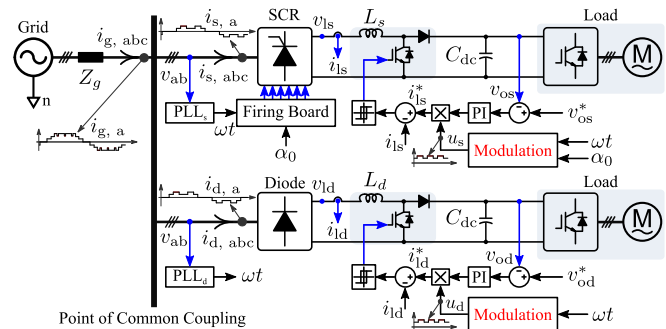
Fig. 1. Schematic and control structure of a multidrive system with boost converters as the dc-link, where hysteresis current controllers are employed: (PLL—Phase Locked Loop; PI—Proportional Integrator).
