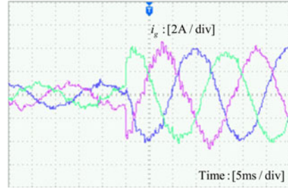
Fig. 20. Experimental transient response of ICF with \lambda = 0.5 , f_s = 4f_{res} .
