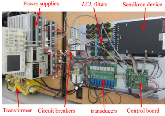
Fig. 17. Three-phase LCL -filtered grid-connected inverter system used in the experimental verification of the delay-dependent stability.
