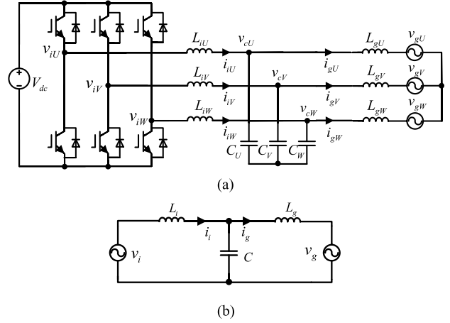
Fig. 1. Three-phase grid-connected inverter with LCL filters. (a) Power circuit. (b) Equivalent single-phase circuit.
