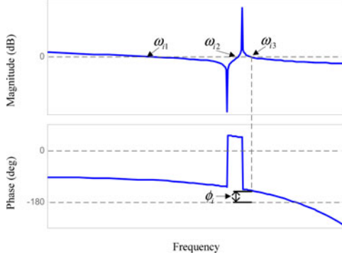
Fig. 9. Bode diagram of the ICF loop gain with time delay in the optimal range.
