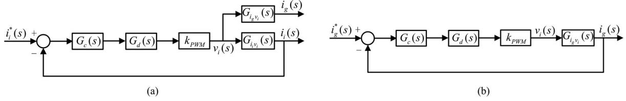
Fig. 3. s -domain block diagrams of the single-loop controlled grid-connected inverters. (a) ICF. (b) GCF.
