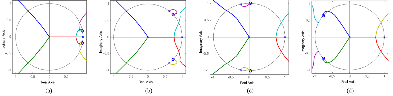
Fig. 7. Root loci of the ICF loop when \lambda = 3 and with T_s in different ranges. (a) T_s \in (0, \pi/7\omega_{\text{res}}) . (b) T_s \in (\pi/7\omega_{\text{res}}, 3\pi/7\omega_{\text{res}}) . (c) T_s \in (3\pi/7\omega_{\text{res}}, 5\pi/7\omega_{\text{res}}) . (d) T_s \in (5\pi/7\omega_{\text{res}}, \pi/\omega_{\text{res}}) .
