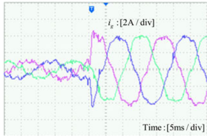
Fig. 26. Experimental transient response of GCF with \lambda = 0.5 , f_s = 6f_{res} , a delay of 2T_s added.
