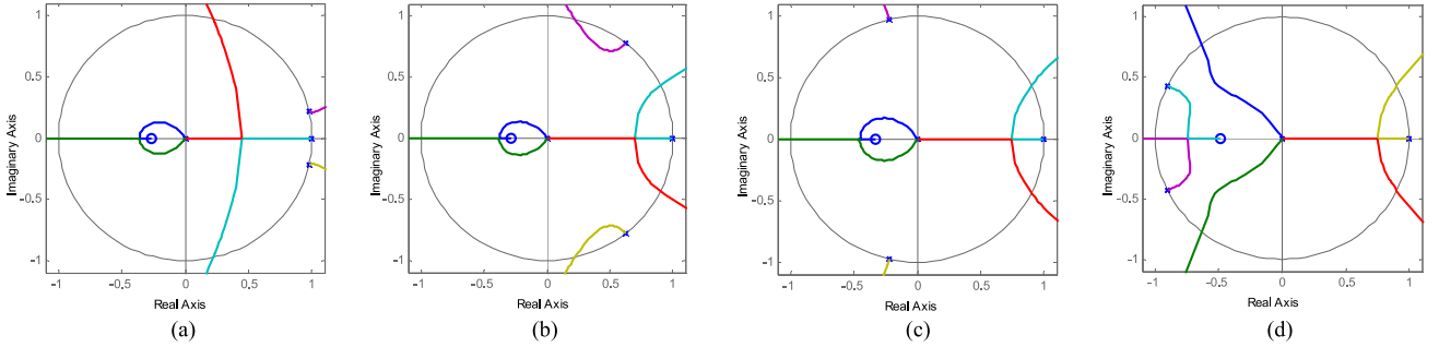
Fig. 8. Root loci of the GCF loop when \lambda = 3 and with T_s in different ranges. (a) T_s \in (0, \pi/7\omega_{\text{res}}) . (b) T_s \in (\pi/7\omega_{\text{res}}, 3\pi/7\omega_{\text{res}}) . (c) T_s \in (3\pi/7\omega_{\text{res}}, 5\pi/7\omega_{\text{res}}) . (d) T_s \in (5\pi/7\omega_{\text{res}}, \pi/\omega_{\text{res}}) .
