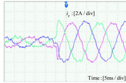
Fig. 29. Experimental transient response of GCF with \lambda = 1 , f_s = 7f_{res} , a delay of 2T_s added.
