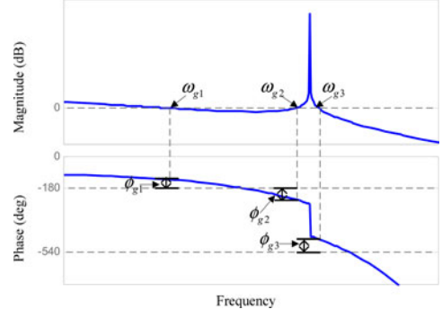
Fig. 10. Bode diagram of the GCF loop gain with time delay in the optimal range.
