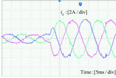
Fig. 23. Experimental transient response of ICF with \lambda = 1 , f_s = 6f_{res} , with linear predictor.
