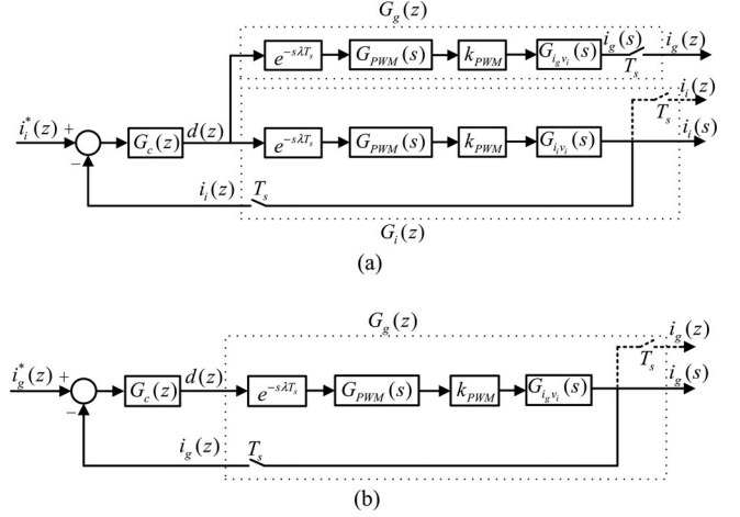
Fig. 6. Block diagrams of the single-loop digitally controlled grid-connected inverters. (a) ICF. (b) GCF.
