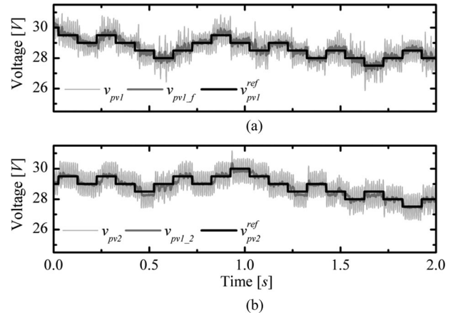
Fig. 7. PV voltage reference v_{pvi}^{ref} (black line) time behavior compared to the measured PV voltage v_{pvi} (light gray line) and to the filtered PV voltage v_{pvi-f} (dark gray line) for the panel #1 (a) and the panel #2 (b), respectively.
