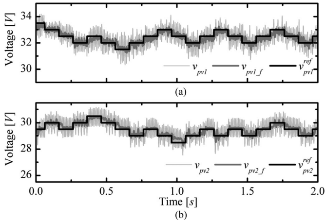
Fig. 12. PV voltage reference v_{pvi}^{ref} (black line) time behavior compared to the measured PV voltage v_{pv} (light gray line) and to the filtered PV voltage v_{pv-f} (dark gray line) for the panel #1 (a) and the panel #2 (b), respectively.
