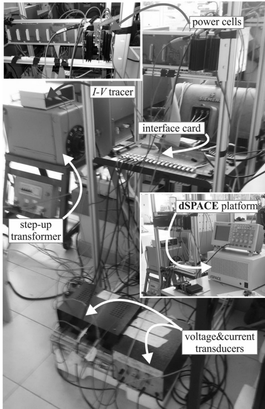
Fig. 5. Laboratory prototype.
