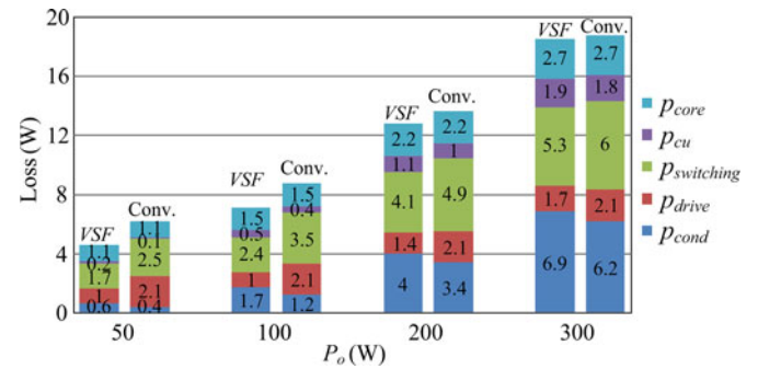
Fig. 14. Loss distribution comparison between proposed VSF and conventional TCM.
