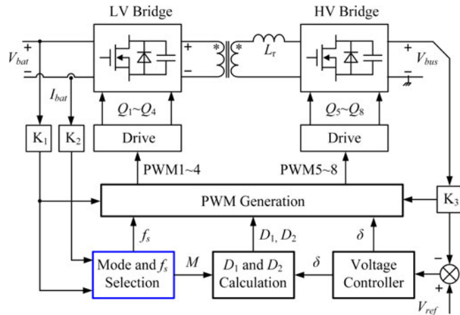
Fig. 27. Control diagram of the DAB converter.
