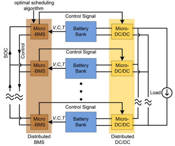
Fig. 7. Block diagram of proposed self-reconfiguration control.
