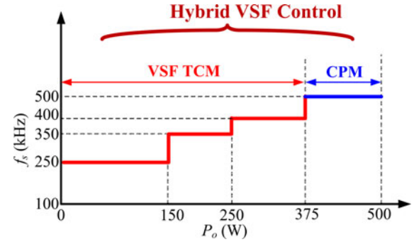
Fig. 10. Proposed VSF hybrid control.
