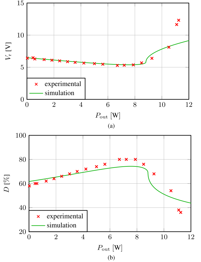
Fig. 7. Comparison of the simulation results with the measured values of the experimental setup. (a) Rectified voltage V_r as a function of the output power P_{out} . (b) Duty cycle D of the dc-dc converter over output power P_{out} .
