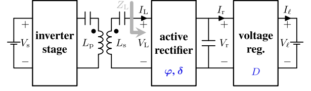
Fig. 1. Schematic block diagram of the overall WPT system including an inverter stage driving the primary side resonance circuit, an active rectifier and a dc-dc converter at the secondary side.
