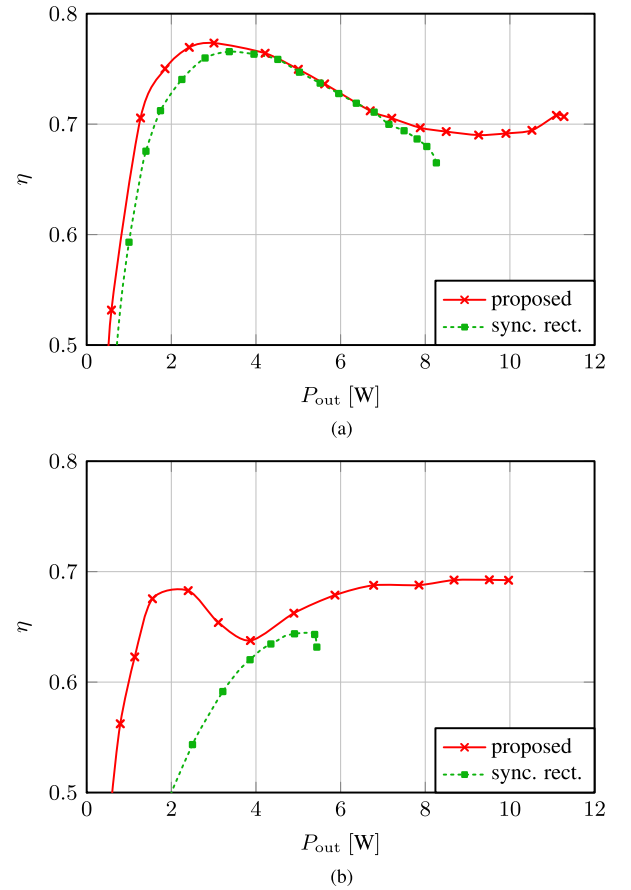
Fig. 10. Experimental results of the overall system efficiency \eta for the proposed concept compared to a synchronous rectifier solution as a function of the output power P_{out} . (a) Measurement results for tightly coupling k = 0.6 . (b) Measurement results for a low coupling factor k = 0.3 .
