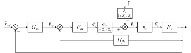
Fig. 7. Additional loop created by output-voltage feedback.
