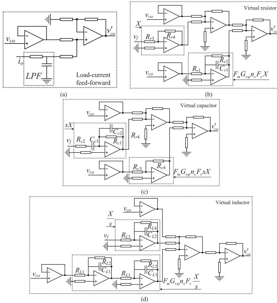
Fig. 19. Practical implementation of output-impedance shaping circuit for: (a) load-current feed-forward; (b) virtual resistor; (c) virtual capacitor; and (d) virtual inductor.
