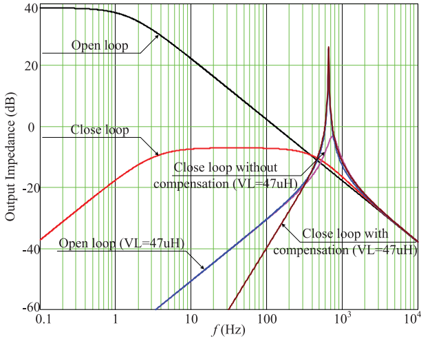
Fig. 17. Plots of converter's open-loop and closed-loop output impedance with/without virtual-inductor implementation and with/without forward-path-gain compensation.
