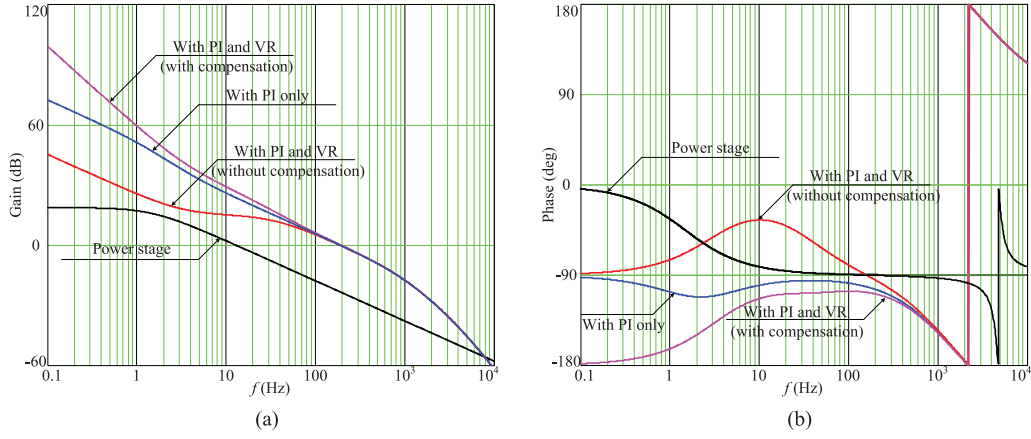
Fig. 10. Bode plots of converter's loop gain with/without virtual-resistor implementation and with/without forward-path-gain compensation.
