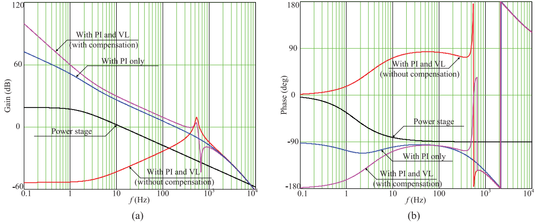
Fig. 16. Bode plots of converter's loop gain with/without virtual-inductor implementation and with/without forward-path-gain compensation.
