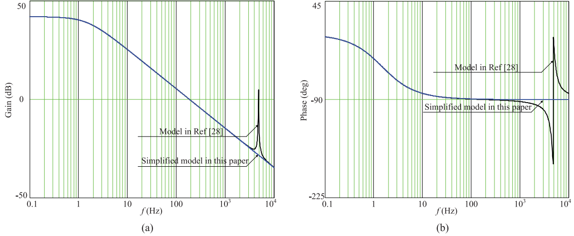
Fig. 3. Bode plots of the phase-shift-to-output-voltage transfer function G'_{v\varphi} = G_{v\varphi} / (1 + Z_o/Z_L) .
