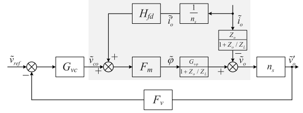
Fig. 5. Additional forward path created by load-current feed-forward.
