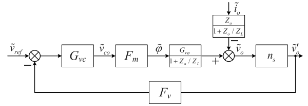
Fig. 4. Basic control system of the converter used in the energy storage branch.
