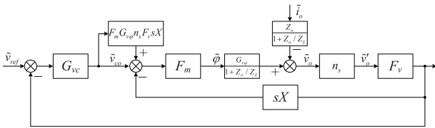
Fig. 12. Control system of the converter used in the energy storage branch implemented with virtual capacitor.
