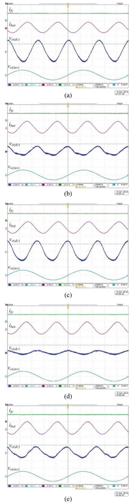
Fig. 21. Static converter waveforms with: (a) PI only; (b) PI and load-current feed-forward; (c) PI and virtual resistor; (d) PI and virtual capacitor; and (e) PI and virtual inductor.
