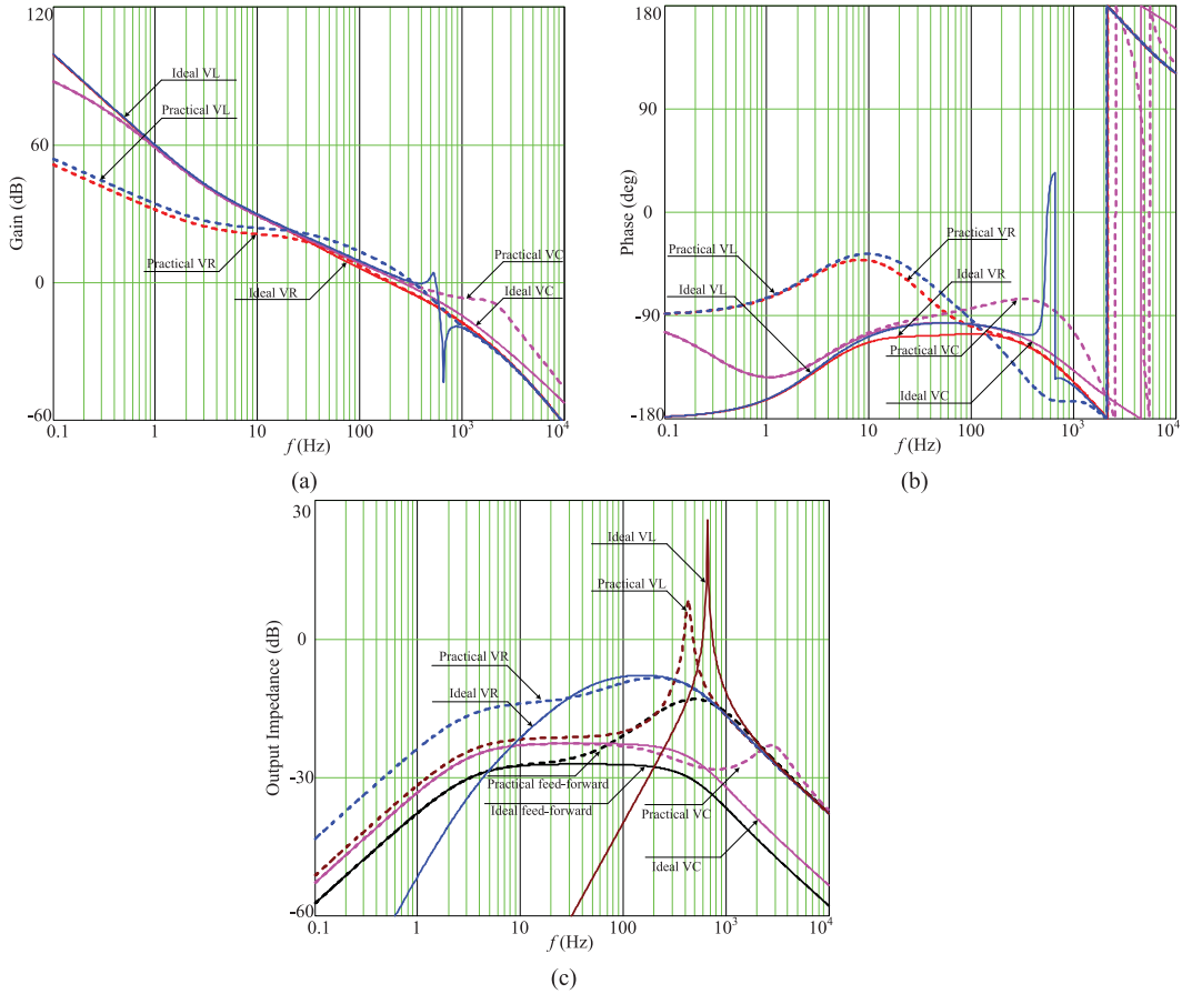
Fig. 20. Bode plots of converter's loop gain and output impedance with ideal and practical implementations of various output-impedance shaping methods: (a) magnitude; (b) phase; and (c) closed-loop output impedance.
