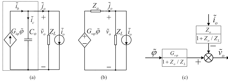
Fig. 2. Approximate small-signal model of bidirectional DAB converter. (a) Norton equivalent circuit. (b) Thevenin equivalent circuit. (c) Transfer-function representation.
