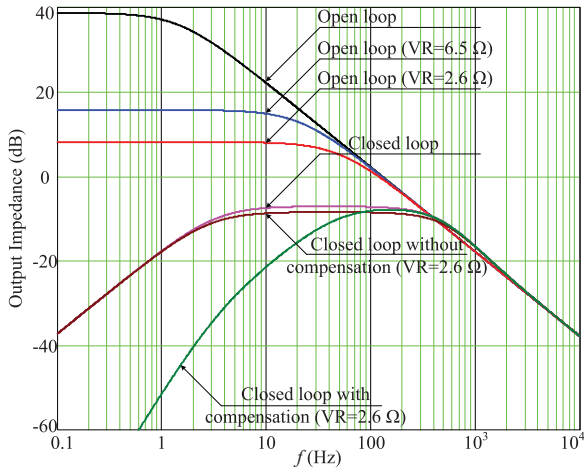
Fig. 11. Plots of converter's open-loop and closed-loop output impedance with/without virtual-resistor implementation and with/without forward-path-gain compensation.
