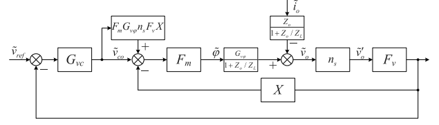
Fig. 9. Control system of the converter used in the energy storage branch implemented with virtual resistor.
