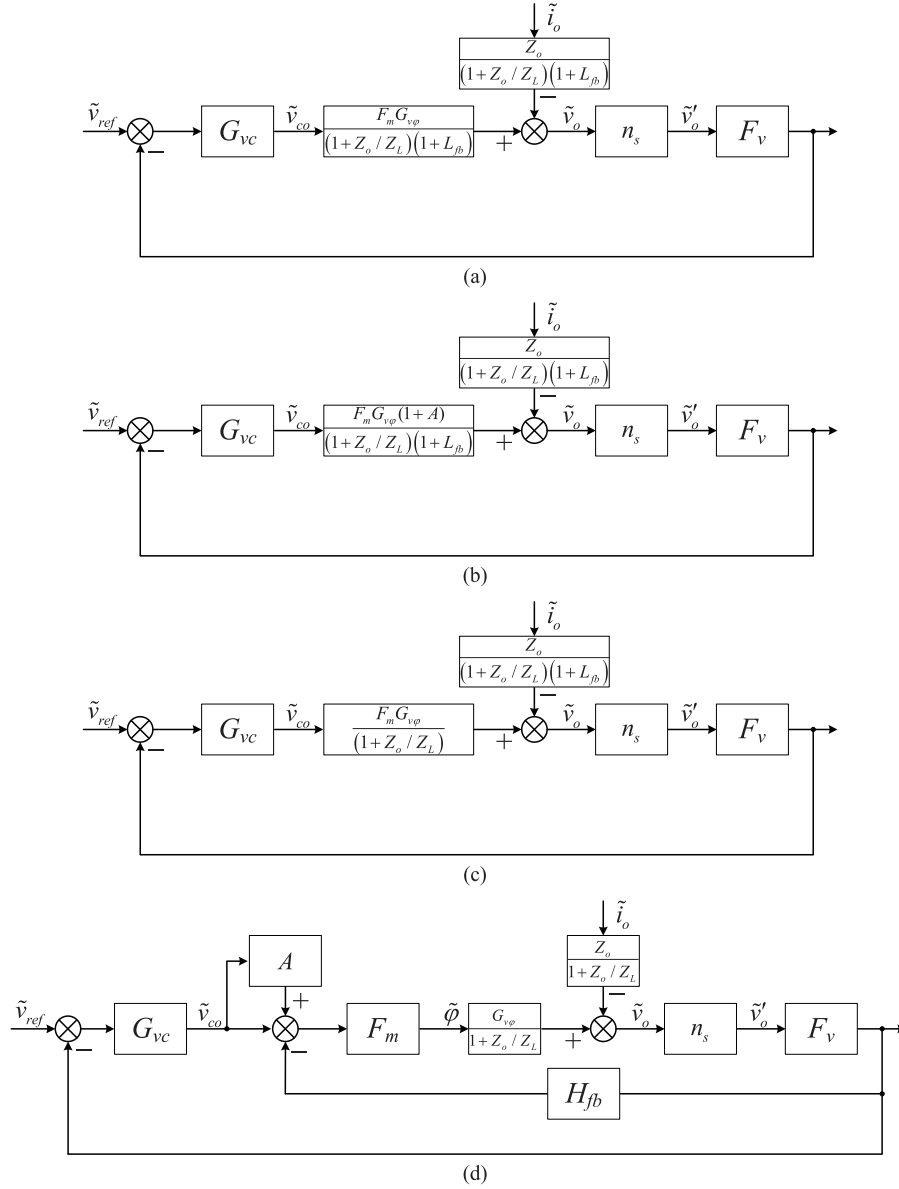
Fig. 8. Derivation of method for compensating the effect of additional loop L_{fb} on converter's dynamic response.
