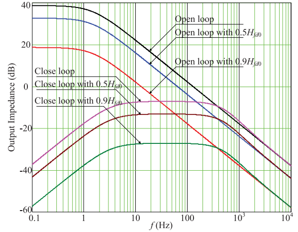
Fig. 6. Open-loop and closed-loop output impedance with and without load-current feed-forward.
