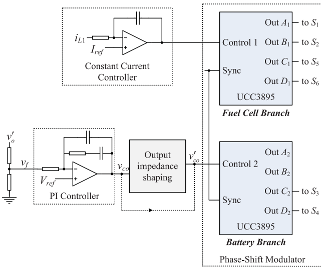
Fig. 18. Practical controller's design for a two-input bidirectional DAB dc-dc converter system.
