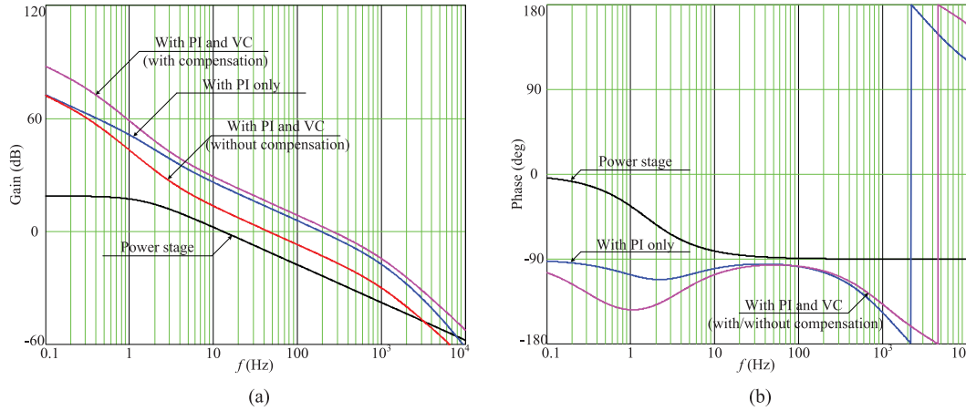
Fig. 13. Bode plots of converter's loop gain with/without virtual-capacitor implementation and with/without forward-path-gain compensation.
