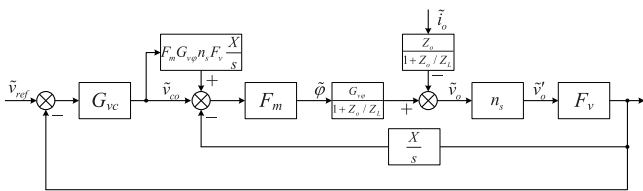
Fig. 15. Control system of the converter used in the energy storage branch implemented with virtual inductor.
