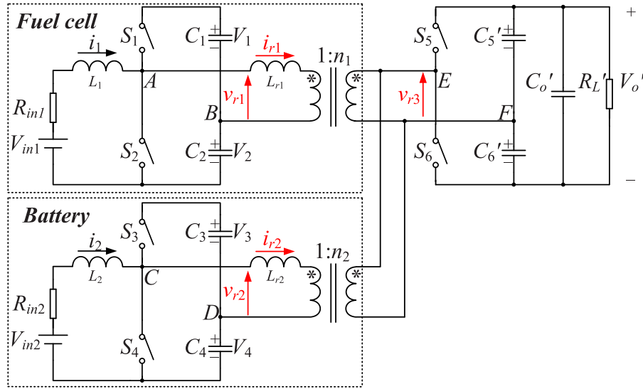
Fig. 1. Multiinput bidirectional DAB dc-dc converter with shared secondary half-bridge cell.
