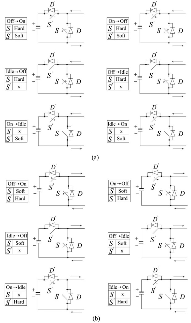
Fig. 10. All possible state transitions of a half-bridge Q2LC cell with (a) Positive (charging) current, and (b) Negative (discharging) current.
