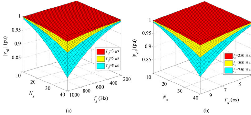
Fig. 7. Fundamental output voltage of the Q2LC in terms of N , \omega_s , and T_d . (a) For discrete values of T_d and (b) discrete values of \omega_s .
