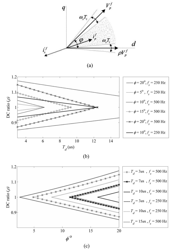
Fig. 11. (a) Phasor diagram representing ac voltages and currents of a Q2LC-based DAB. [Superscript f denotes fundamental component]. (b) equation (25) plotted against dwell time, and (c) equation (25) plotted against load angle.
