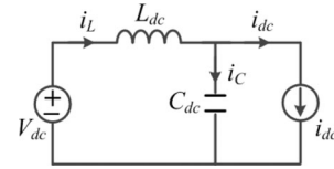
Fig. 2. Equivalent circuit of dc-link.
