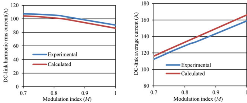
Fig. 8. Experimental and calculated comparison results with balanced load.
