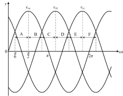
Fig. 3. Three-phase reference signals.
