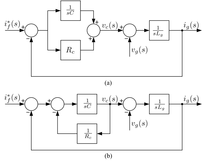
Fig. 2. s -domain block diagram representations of an LCL -filter with a damping resistor (a) in series with and (b) in parallel with the capacitor.
