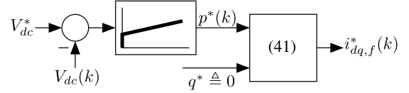
Fig. 4. Fundamental dq -frame converter current reference generation for model predictive direct current control.
