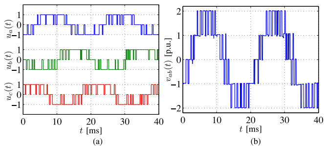
Fig. 9. Experimental (a) switching states and (b) line-to-line converter voltage.
