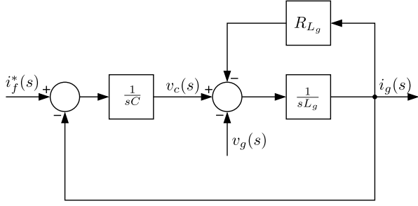
Fig. 3. s -domain block diagram representation of an LCL -filter with a resistor R_{L_g} in series with the grid-side inductor.
