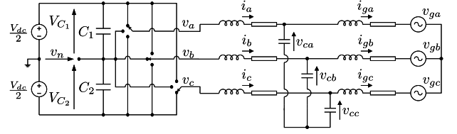
Fig. 1. Representation of a three-phase NPC converter connected to the grid via an LCL -filter.
