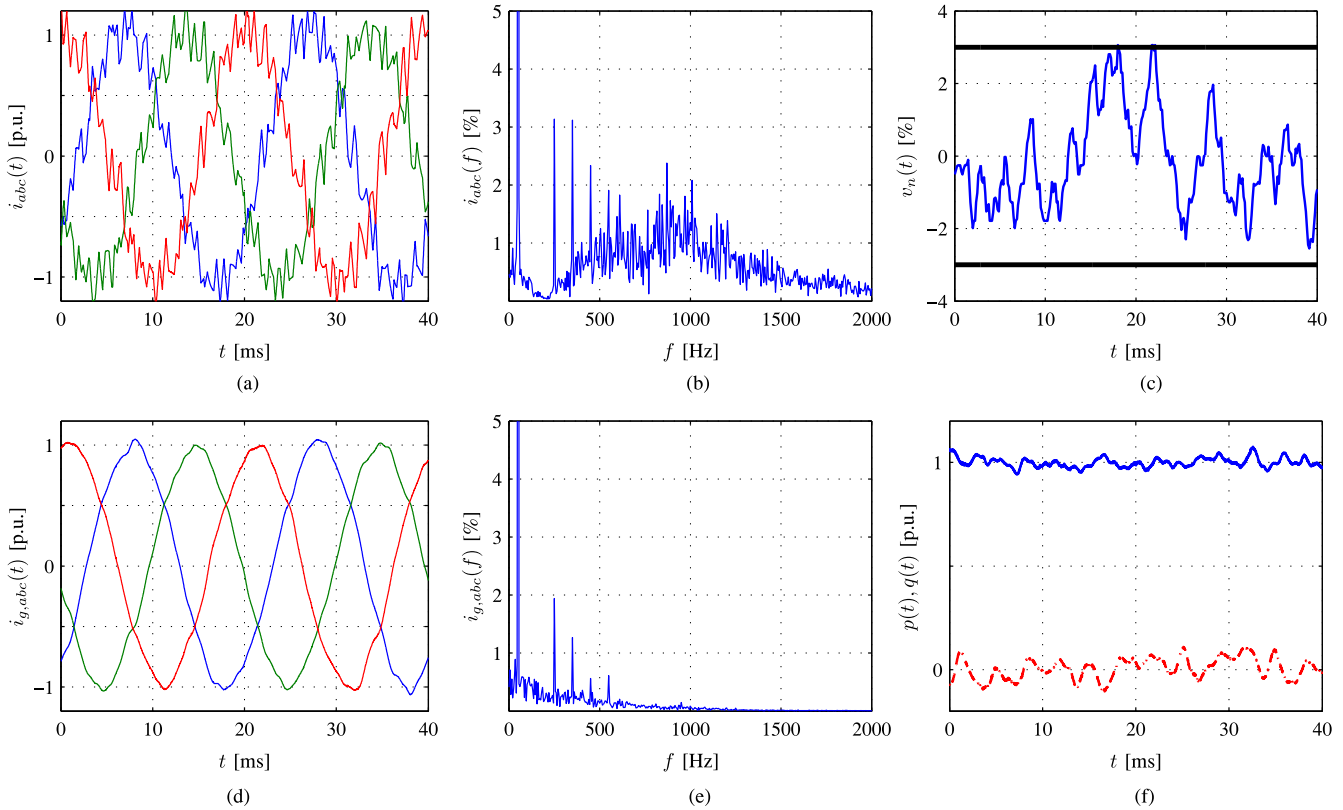
Fig. 10. Experimental (a) converter currents, (b) converter current spectrum, (c) neutral-point potential and bounds, (d) grid currents, (e) grid current spectrum, and (f) real and reactive power, for the proposed MPDCC-VR strategy with N_s = \text{“eSE.”}
