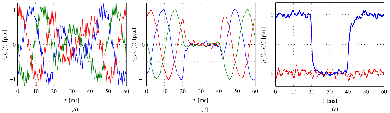
Fig. 11. Experimental (a) converter currents, (b) grid currents, and (c) real and reactive power, for the proposed MPDCC-VR strategy under transient conditions with N_s = \text{“eSE.”}
