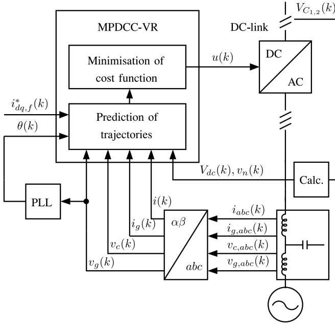
Fig. 5. Setup for MPDCC-VR for a three-phase NPC connected to the grid via an LCL -filter.
