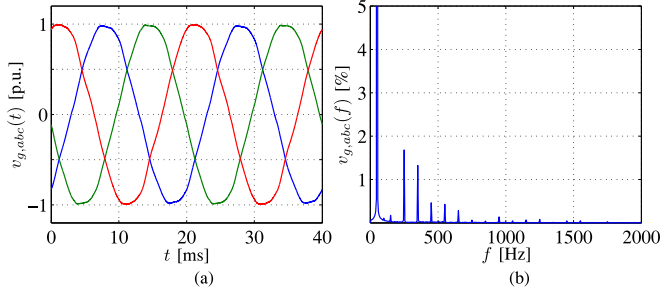
Fig. 8. Experimental (a) grid voltages and (b) spectrum.
