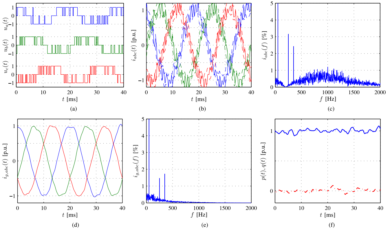
Fig. 7. Simulated (a) switching states, (b) converter currents and bounds, (c) converter current spectrum, (d) grid currents, (e) grid current spectrum, and (f) real (blue, solid) and reactive (red, dashed) power, for the proposed MPDCC-VR strategy with N_s = \text{"eSE"} with harmonic attenuation.
