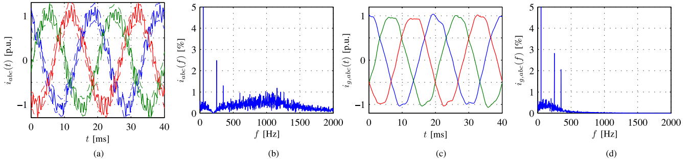
Fig. 6. Simulated (a) converter currents and bounds, (b) converter current spectrum, (c) grid currents, and (d) grid current spectrum, for the proposed MPDCC-VR strategy with N_s = \text{"eSE"} without harmonic attenuation.
