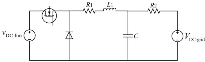
Fig. 10. Grid-tied dc/dc buck converter topology.
