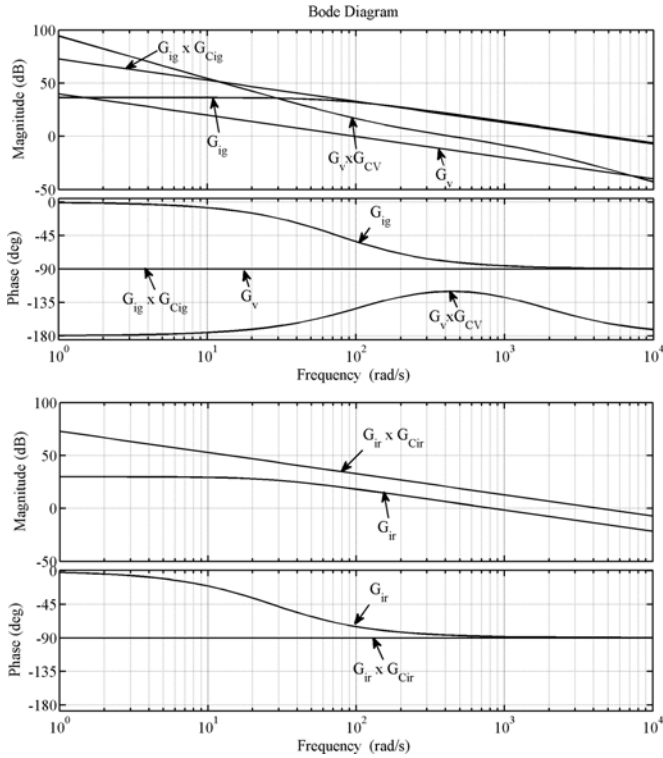
Fig. 7. Bode plots for the designed compensators of VSC 2 and VSC 1 control.
