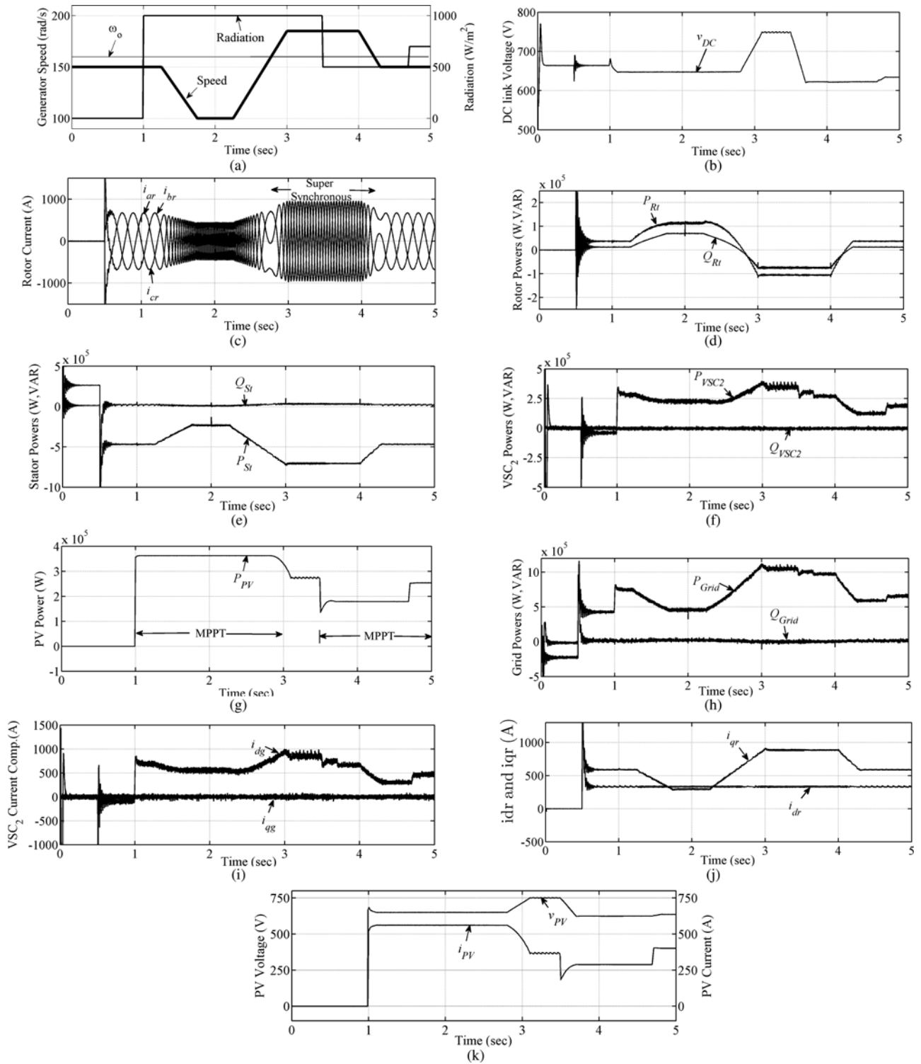
Fig. 9. Simulation results for: (a) machine mechanical speed and radiation pattern applied to the hybrid system; (b) dc-link voltage controlled by the algorithm (see Fig. 5) via VSC 2 ; (c) rotor current performance under different machine speeds; (d), (e) active and reactive components of rotor and stator power; (f) loading of VSC 2 ; (g) PV power generation; (h) power injected into the grid; (i) VSC 2 current components; (j) rotor current components; (k) PV terminal voltage and current.
