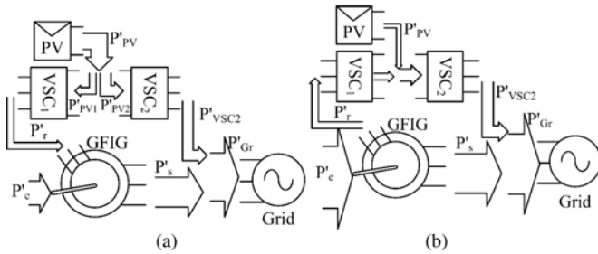
Fig. 8. Power conversion process in various segments of the proposed hybrid PV-wind-energy system during most of the day (as per actual power flow direction indicated by P'_r , P'_{VSC2} , etc.). (a) High solar radiation, low wind speed. (b) Low solar radiation (or during nights), high wind speed.
