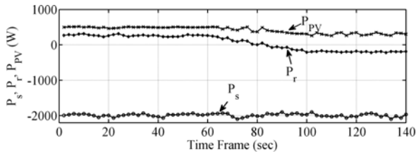
Fig. 13. Experimental results showing stator power, rotor power, and PV power over the complete operating range.
