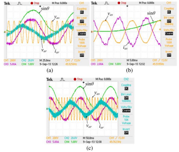
Fig. 12. Experimental results: (a) sub-synchronous operating mode showing A-ph rotor current and voltage, A-phase stator voltage, and sine transformation angle for rotor quantities; (b) sub-synchronous mode showing A-ph stator voltage and current and sine transformation angle; (c) supersynchronous mode showing the same parameters as in (a).
