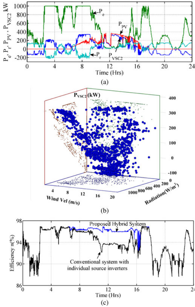
Fig. 10. Simulation results with per minute data provided in Fig. 1(b) over a day for: (a) power flow in various sections ( P_e , P_r , P_{VSC2} , and P_{PV} ); (b) VSC_2 loading in kilowatt; (c) efficiency analysis to compare the benefits of the proposed hybrid system with conventional distributed generation having individual source converters.
