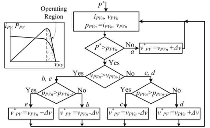
Fig. 5. PV power control algorithm for the proposed hybrid PV-wind system.
