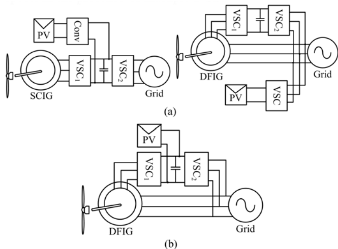
Fig. 2. (a) Block diagram of the conventional PV-wind hybrid systems. (b) Proposed PV-wind hybrid system.
