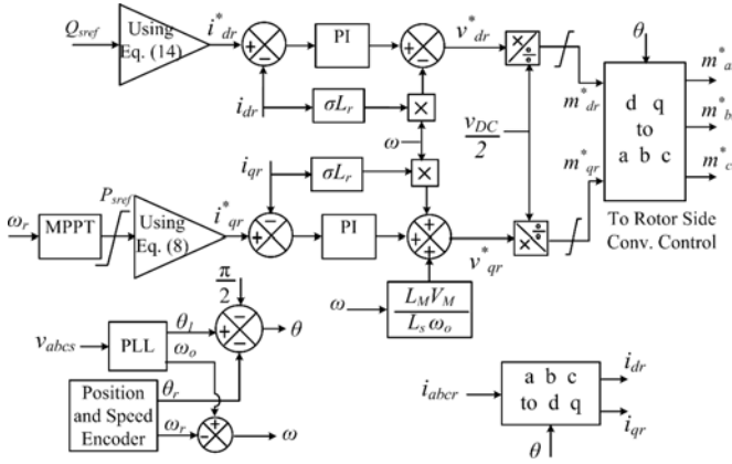
Fig. 4. Rotor-side converter, VSC 1 control.
