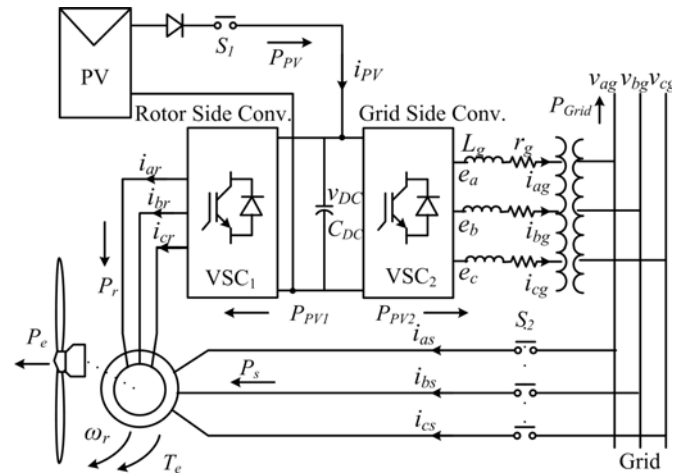
Fig. 3. Proposed solar PV-wind DFIG system.
