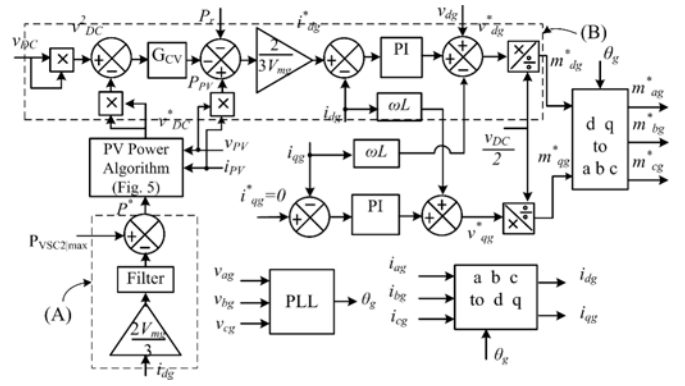
Fig. 6. Proposed control strategy for the grid-side inverter, VSC 2 .
