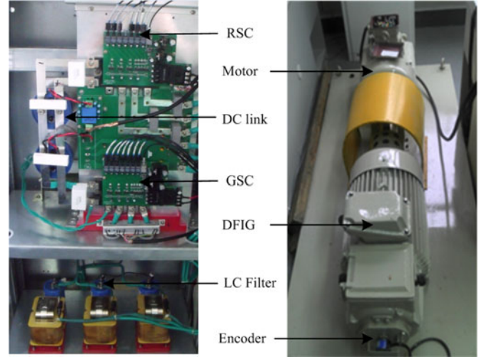
Fig. 8. Experimental setup of the tested DFIG.
